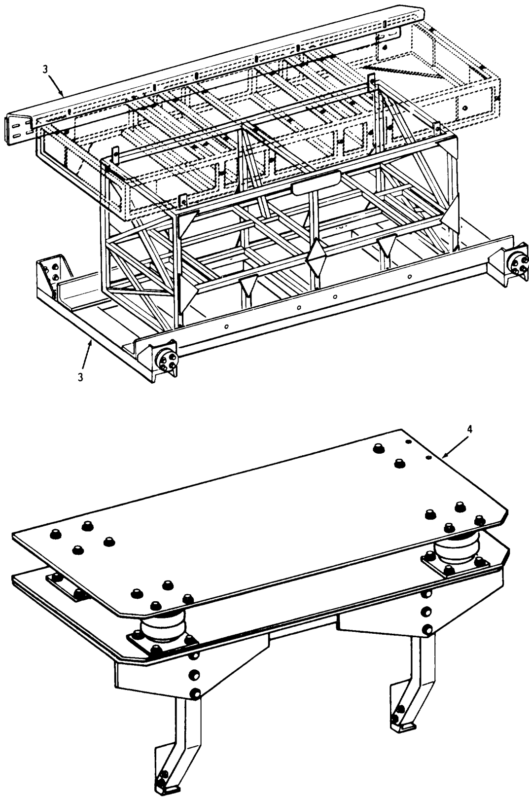
Figure 1. Computer System, Gun Direction AN/GYK-29(V) (Sheet 5 of 5)
