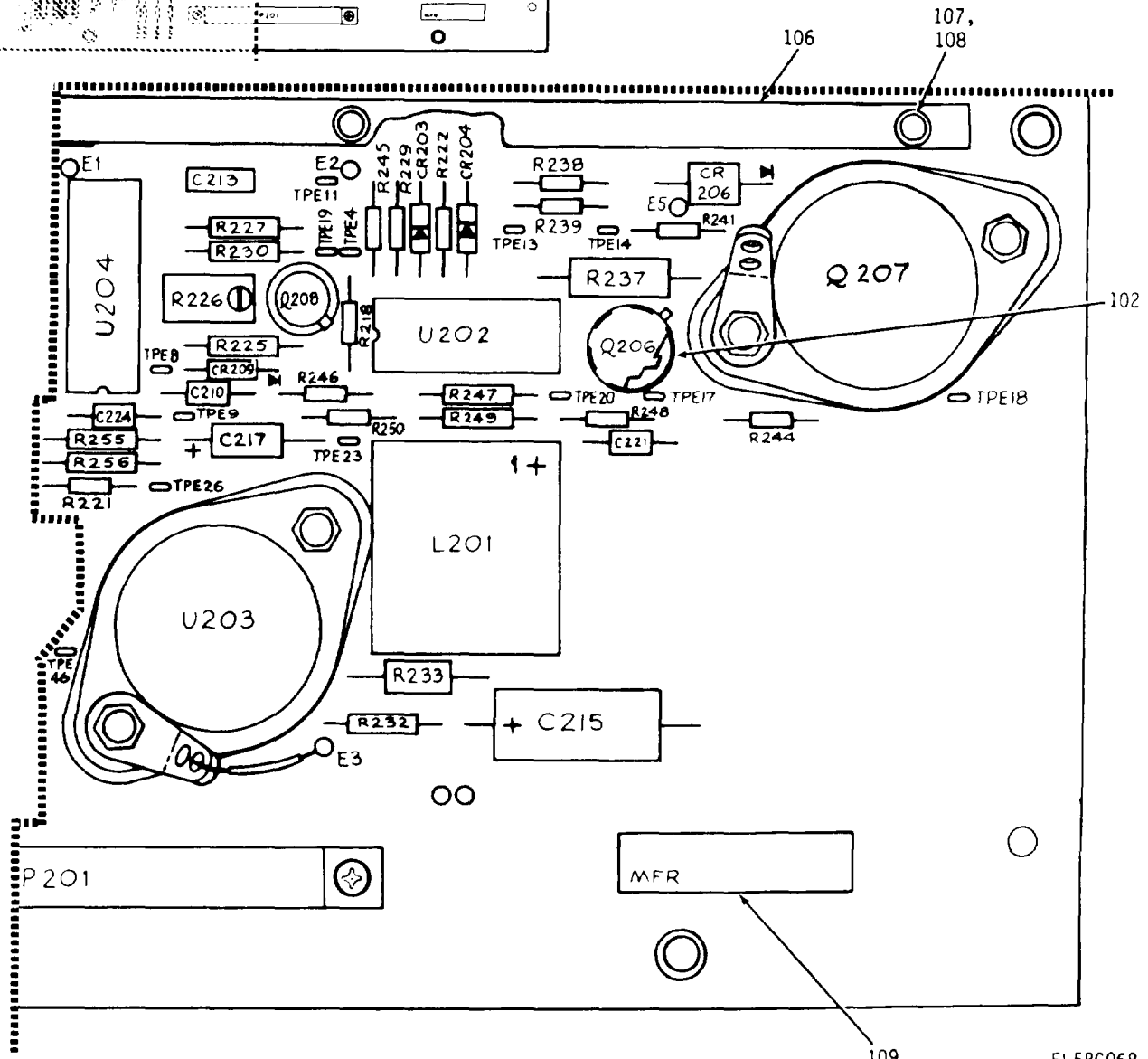
Figure 15. LVPS Backup Board Assembly (Sheet 4 of 6)
