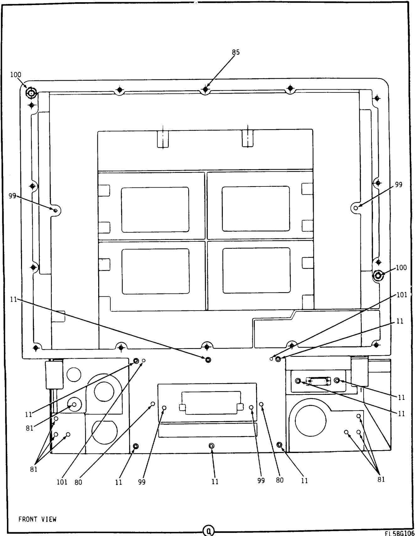
Figure 25. Housing Assembly (Sheet 7 of 7)
