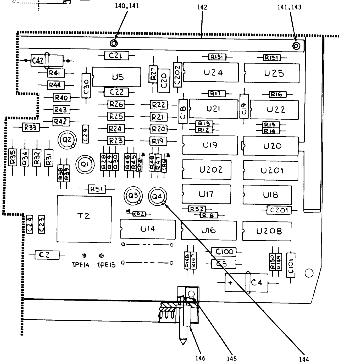
Figure 9. Communication Modem Assembly (Sheet 3 of 6)
