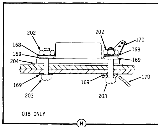
Figure 14. LVPS Main Board Assembly (Sheet 7 of 10)
