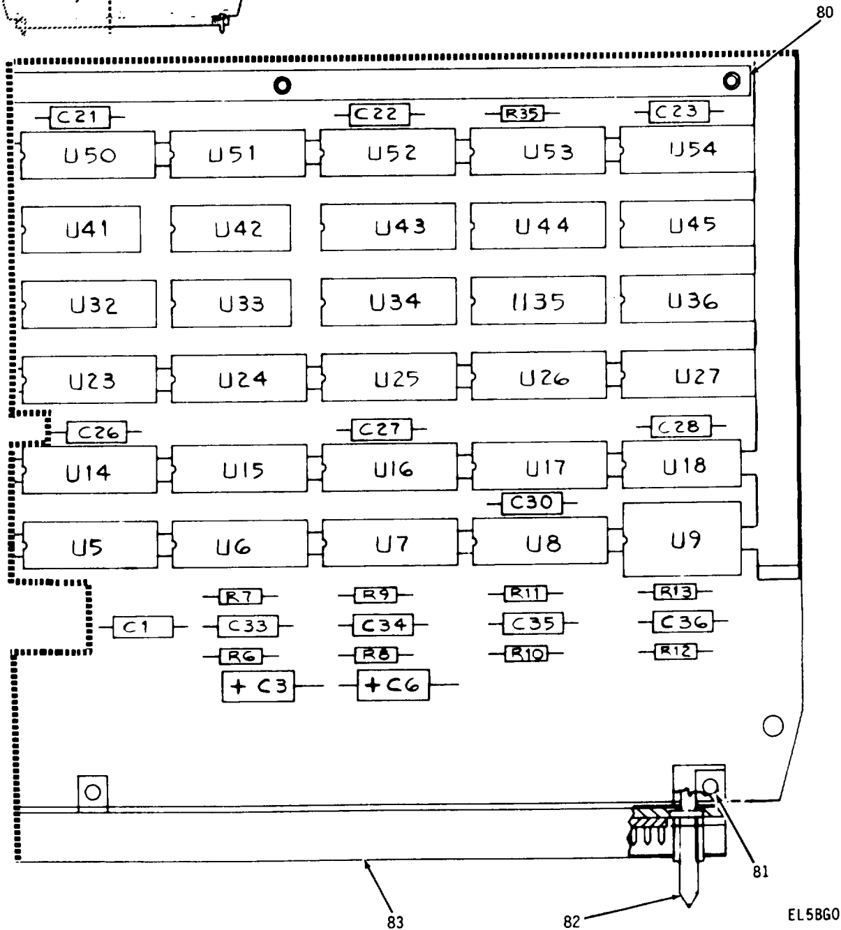
Figure 5. Interface Data Controller 1 Assembly (Sheet 3 of 5)
