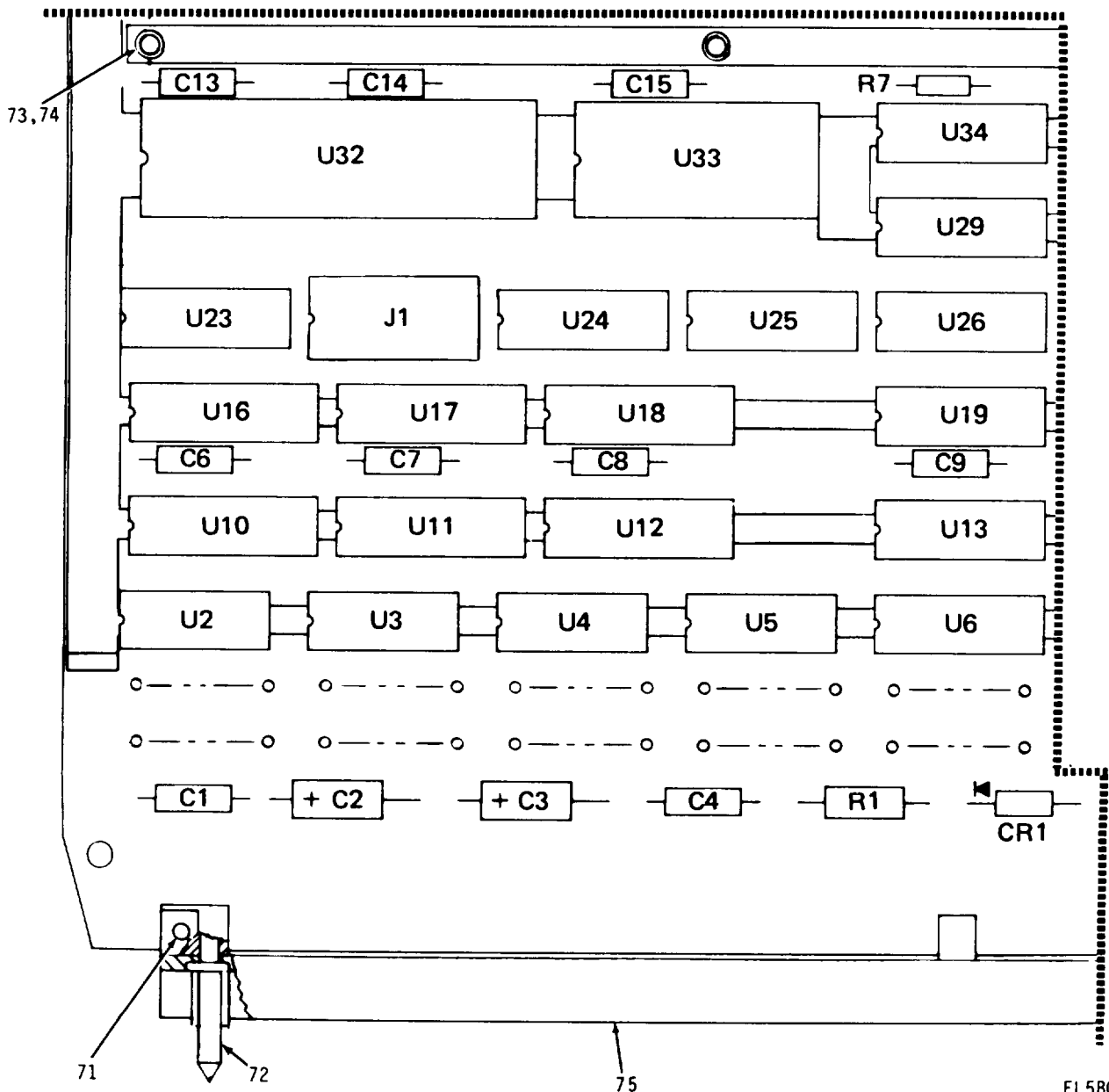
Figure 4. Central Processor Assembly (Sheet 4 of 5)
