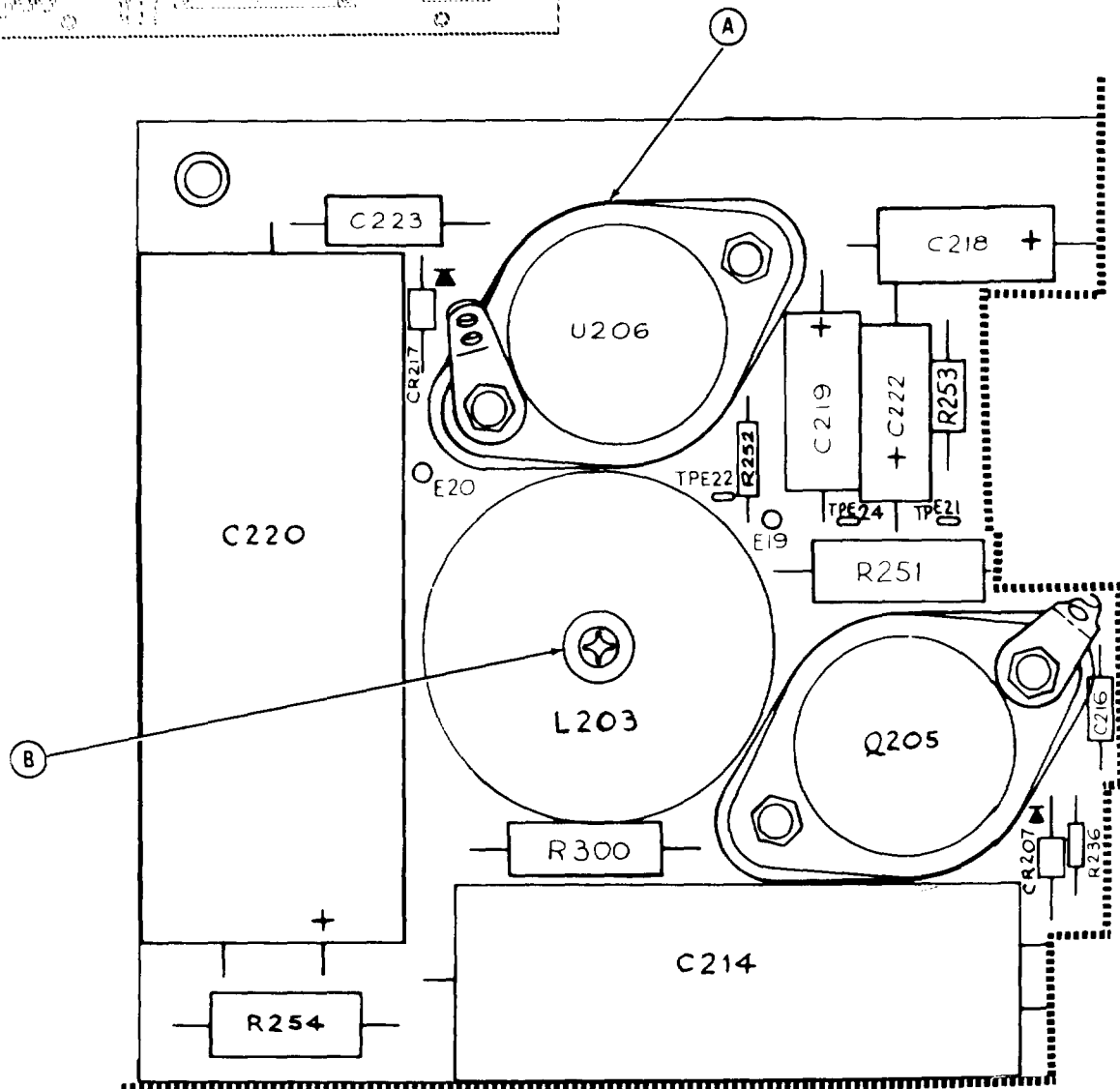
Figure 15. LVPS Backup Board Assembly (Sheet 1 of 6)
