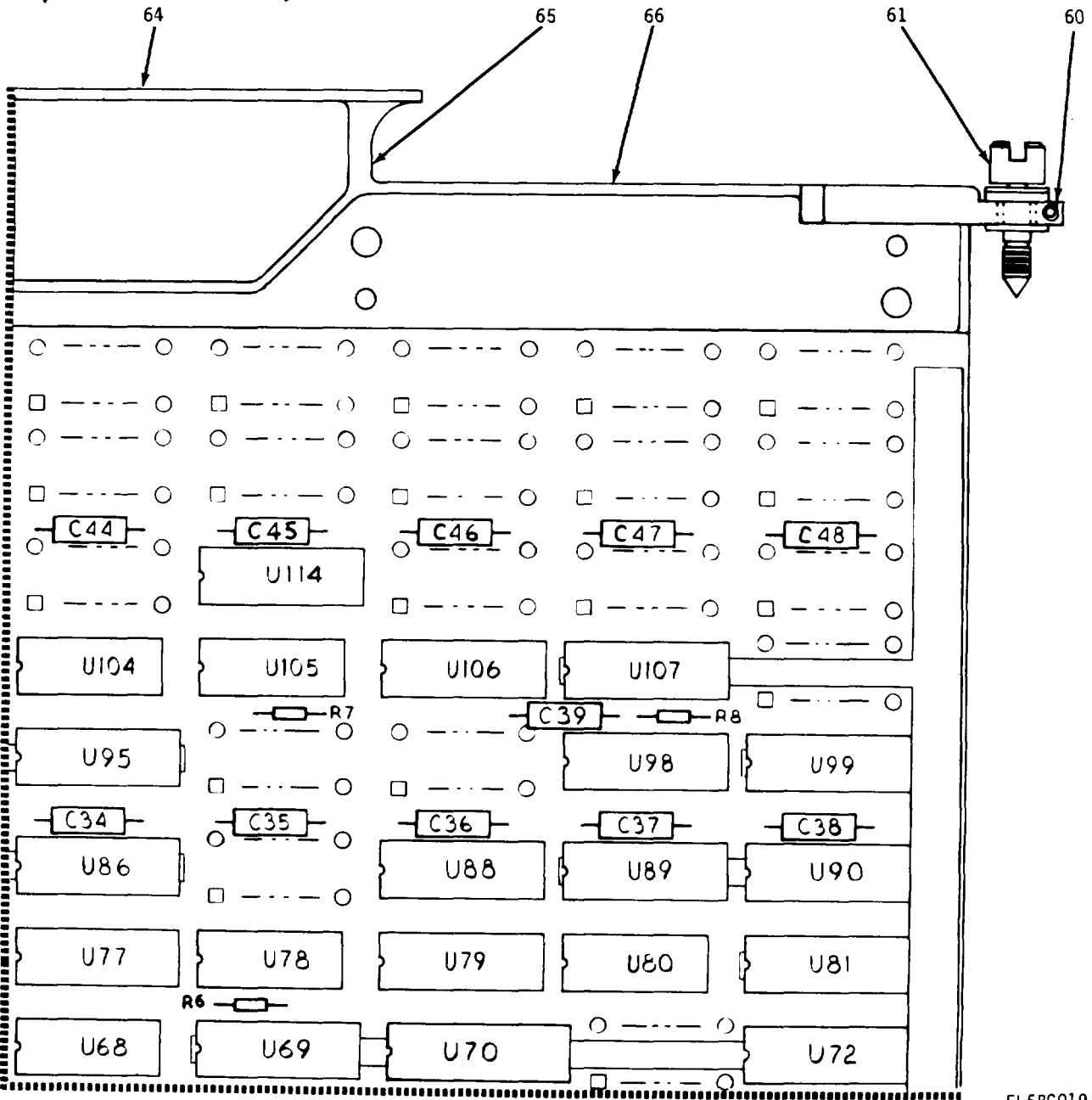
Figure 6. Interface Data Controller 2 Assembly (Sheet 2 of 5)
