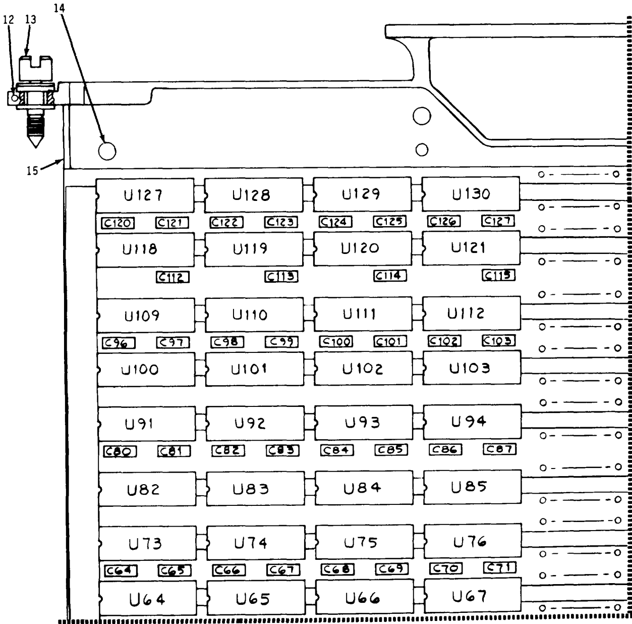
Figure 10. 65 KW Memory Assembly (Sheet 1 of 5)
