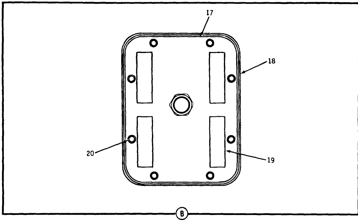
Figure 47. GDU Case Subassembly (Sheet 2 of 2)
