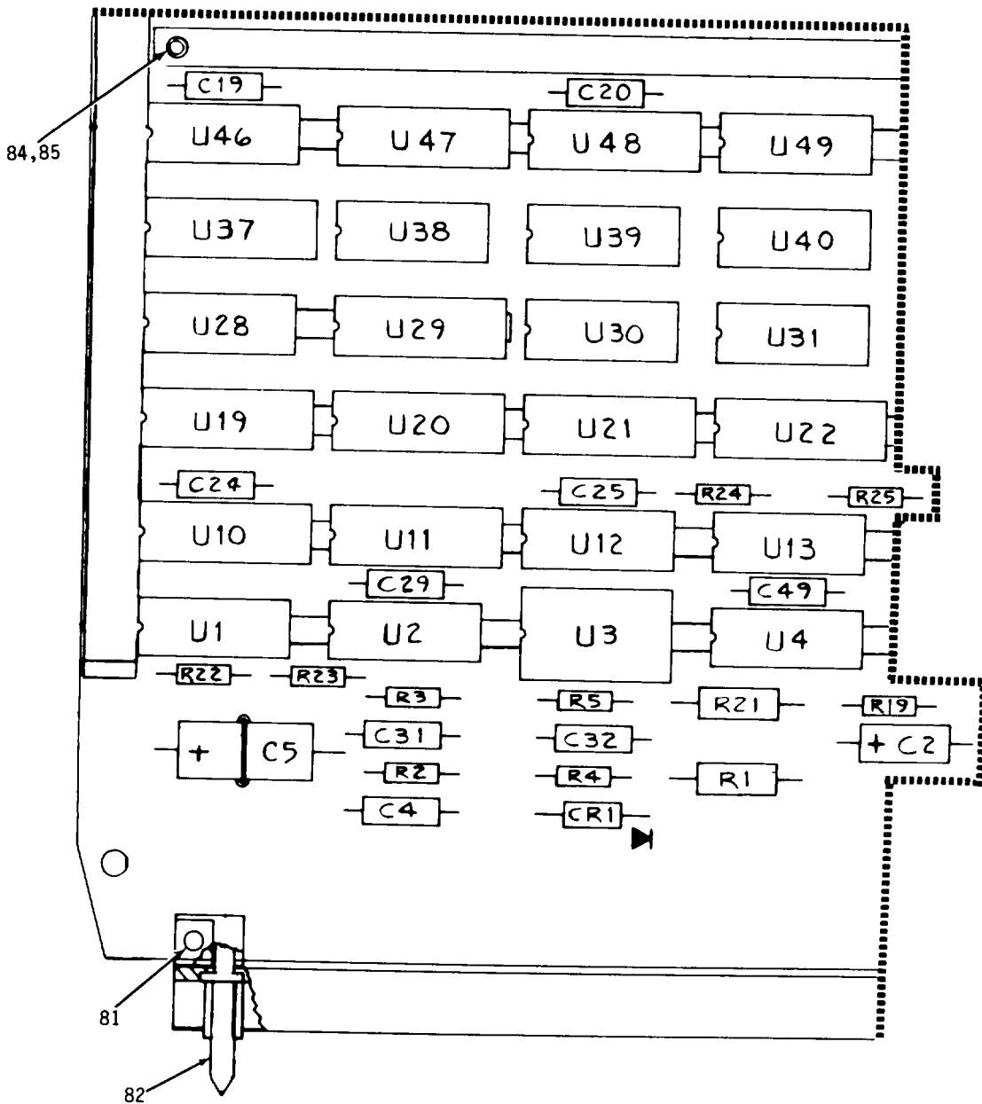
Figure 5. Interface Controller 1 Assembly (Sheet 4 of 5)
