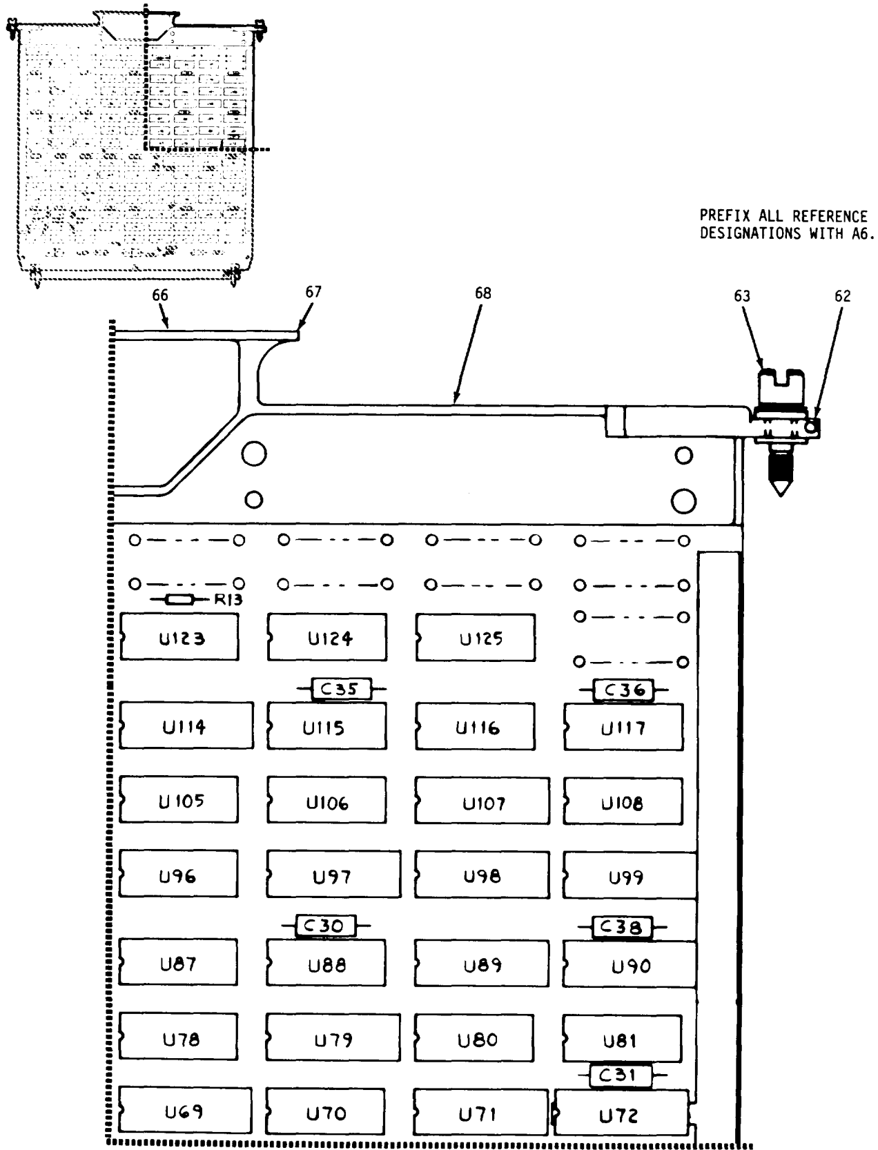
Figure 12. Symbol Generator Assembly (Sheet 2 of 5)
