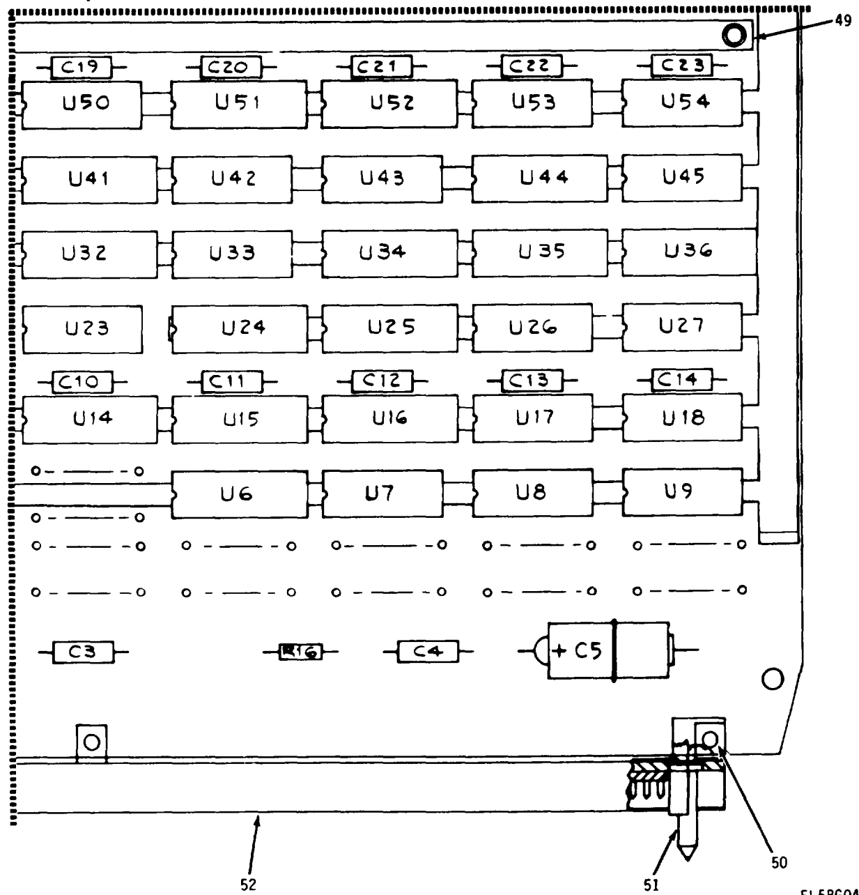
Figure 11. Memory Control Assembly (Sheet 3 of 5)
