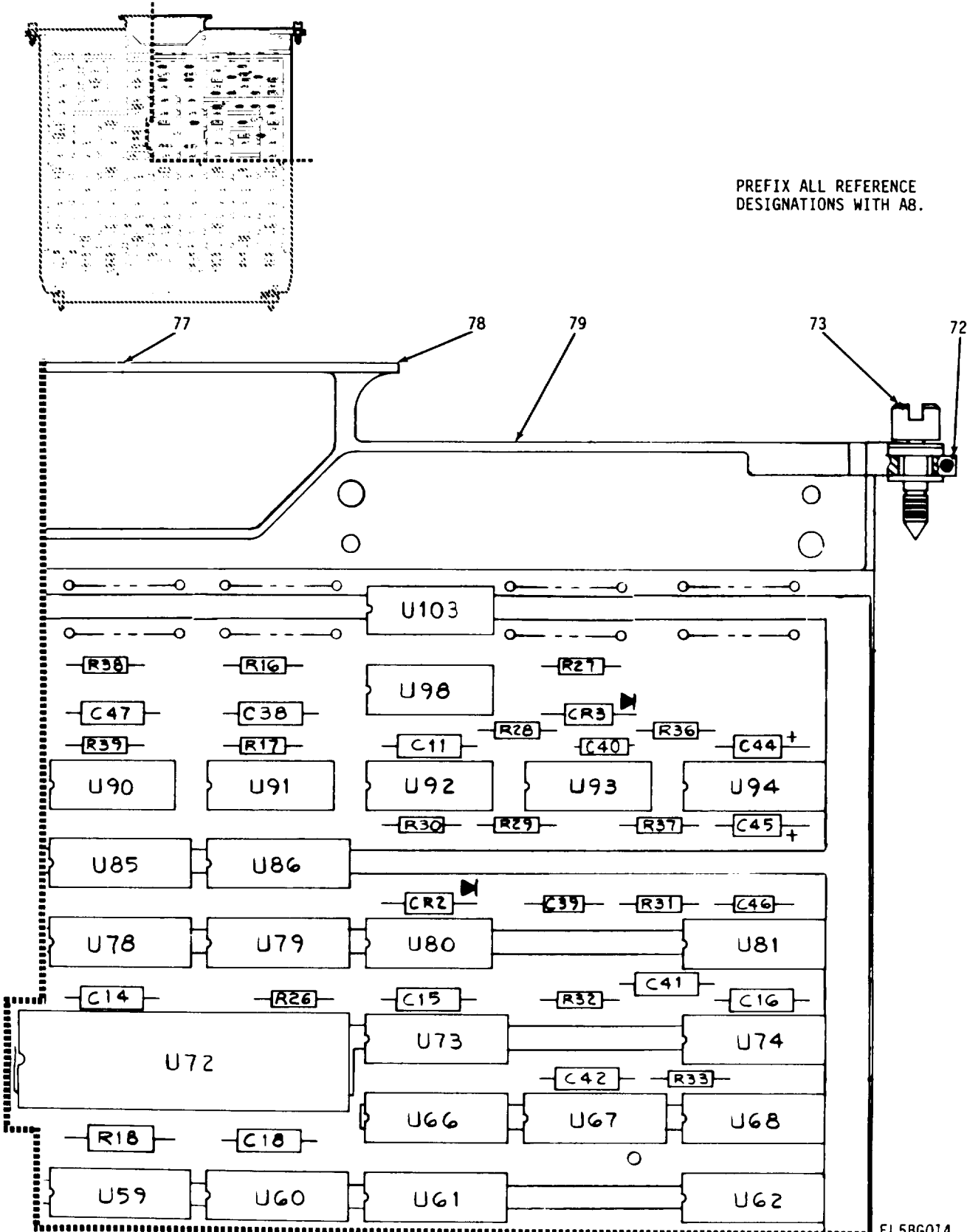
Figure 5. Interface Data Controller 1 Assembly (Sheet 2 of 5)
