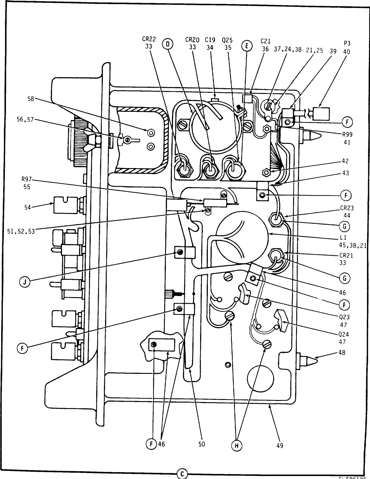
Figure 44. Power Supply Unit Chassis Assembly (Sheet 3 of 4)
