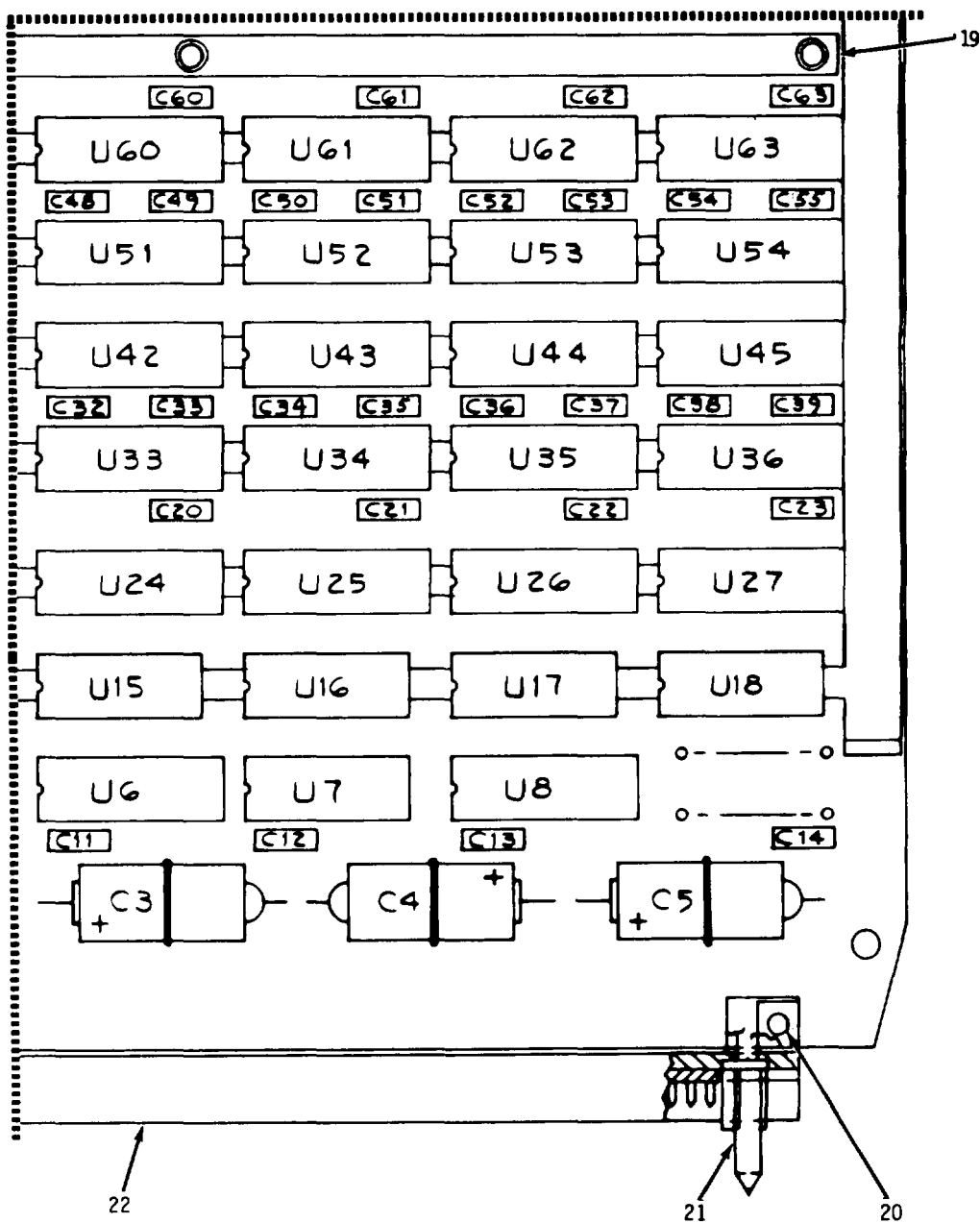
Figure 10. 65 KW Memory Assembly (Sheet 3 of 5)
