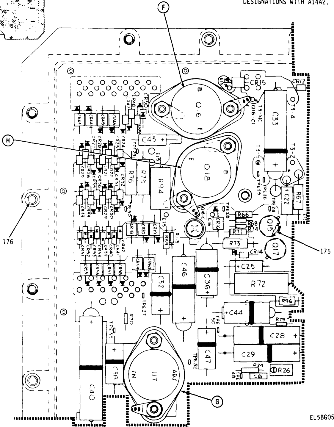
Figure 14. LVPS Main Board Assembly (Sheet 2 of 10)
