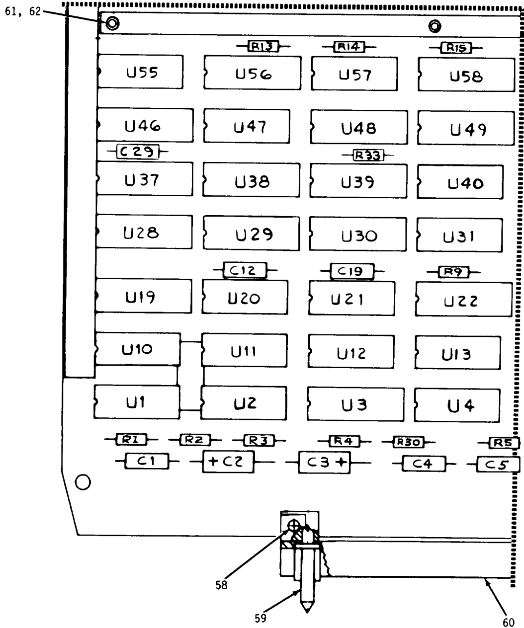
Figure 8. Communication Interface Assembly (Sheet 4 of 5)
