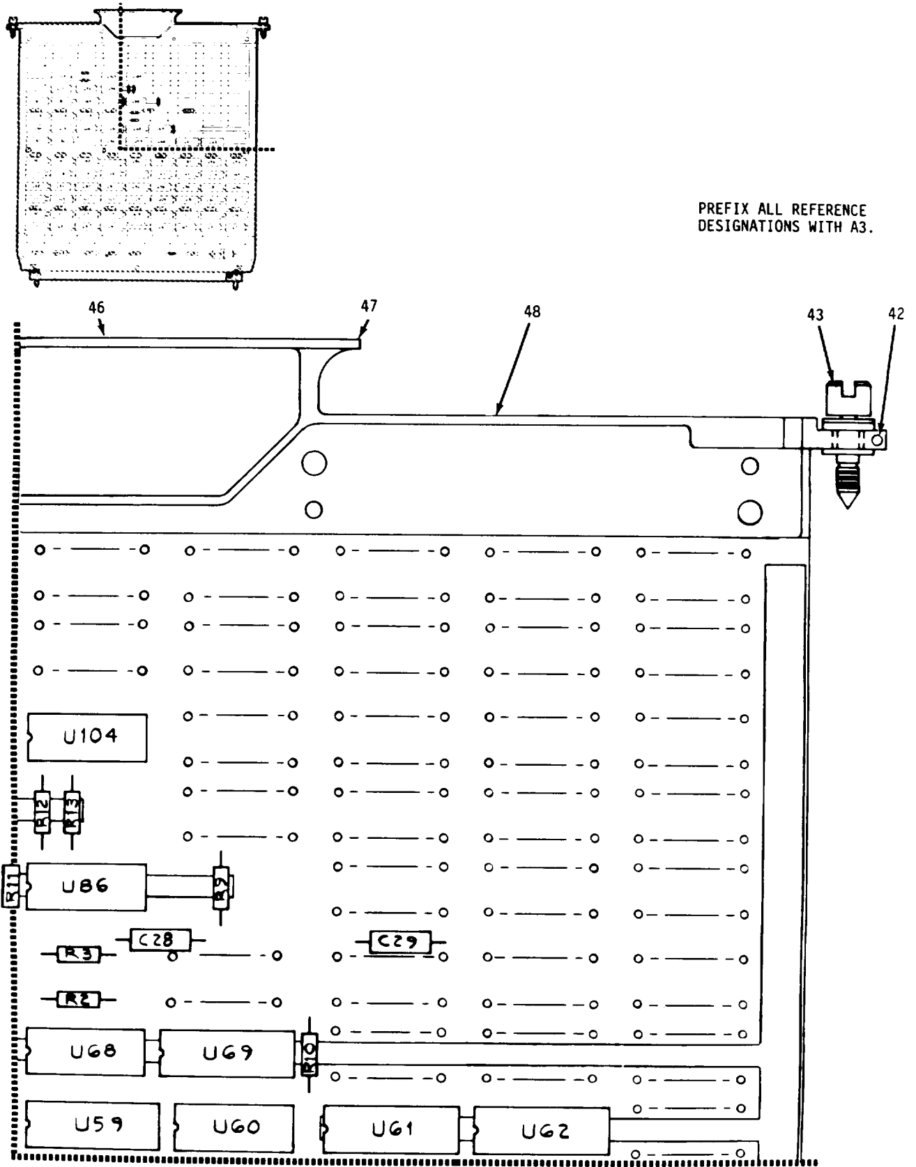
Figure 11. Memory Control Assembly (Sheet 2 of 5)
