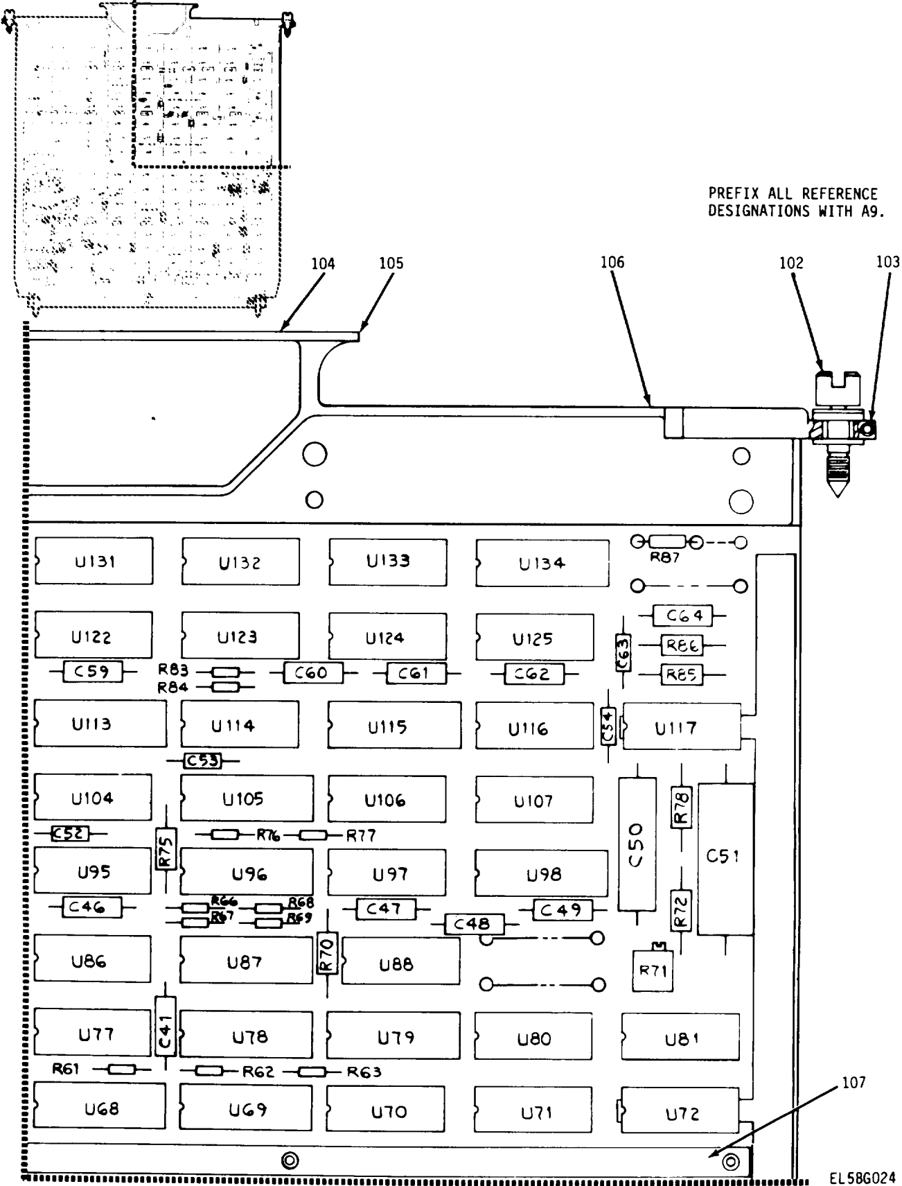
Figure 7. Gun Display Unit interface Assembly (sheet 2 of 5)
