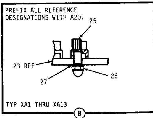
Figure 26. Harness Assembly (Sheet 2 of 2)
