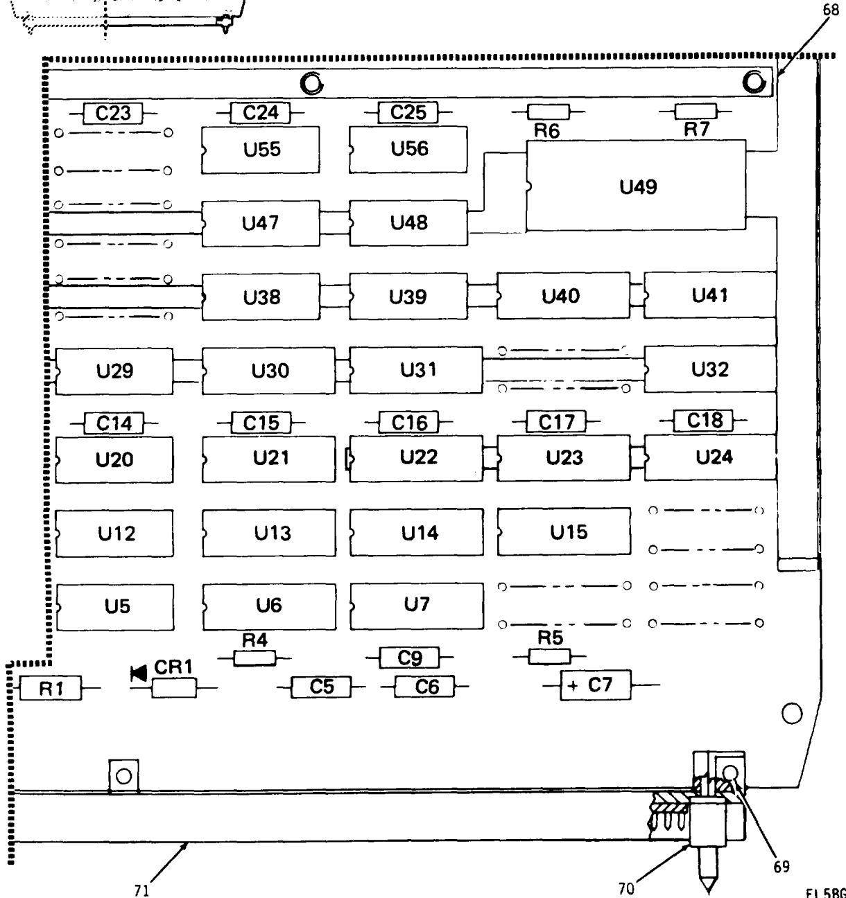
Figure 24. Central Processor Interface Assembly (Sheet 3 of 5)
