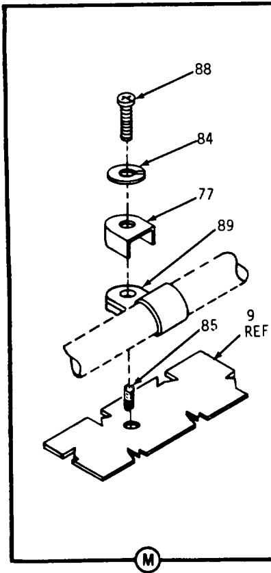
Figure 25. Housing Assembly (Sheet 5 of 7)
