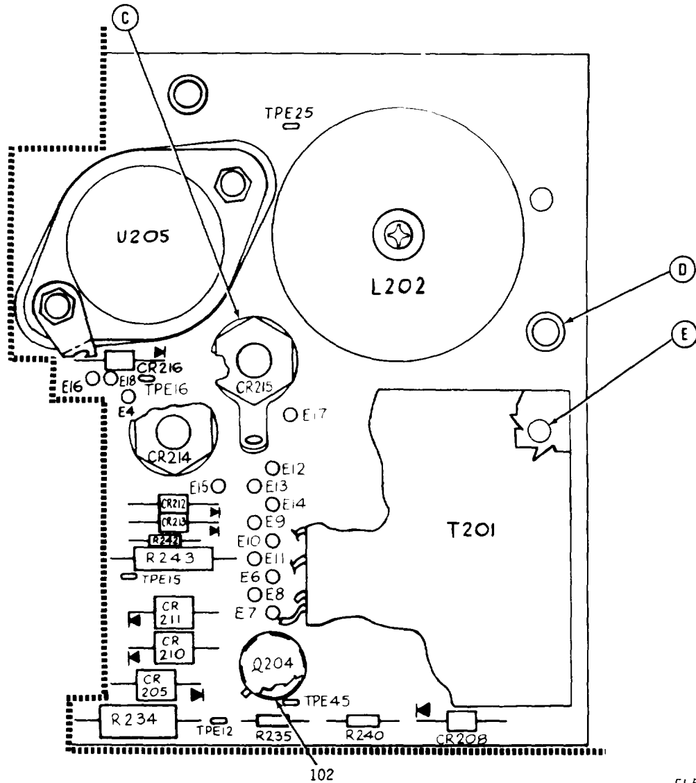
Figure 15. LVPS Backup Board Assembly (Sheet 2 of 6)
