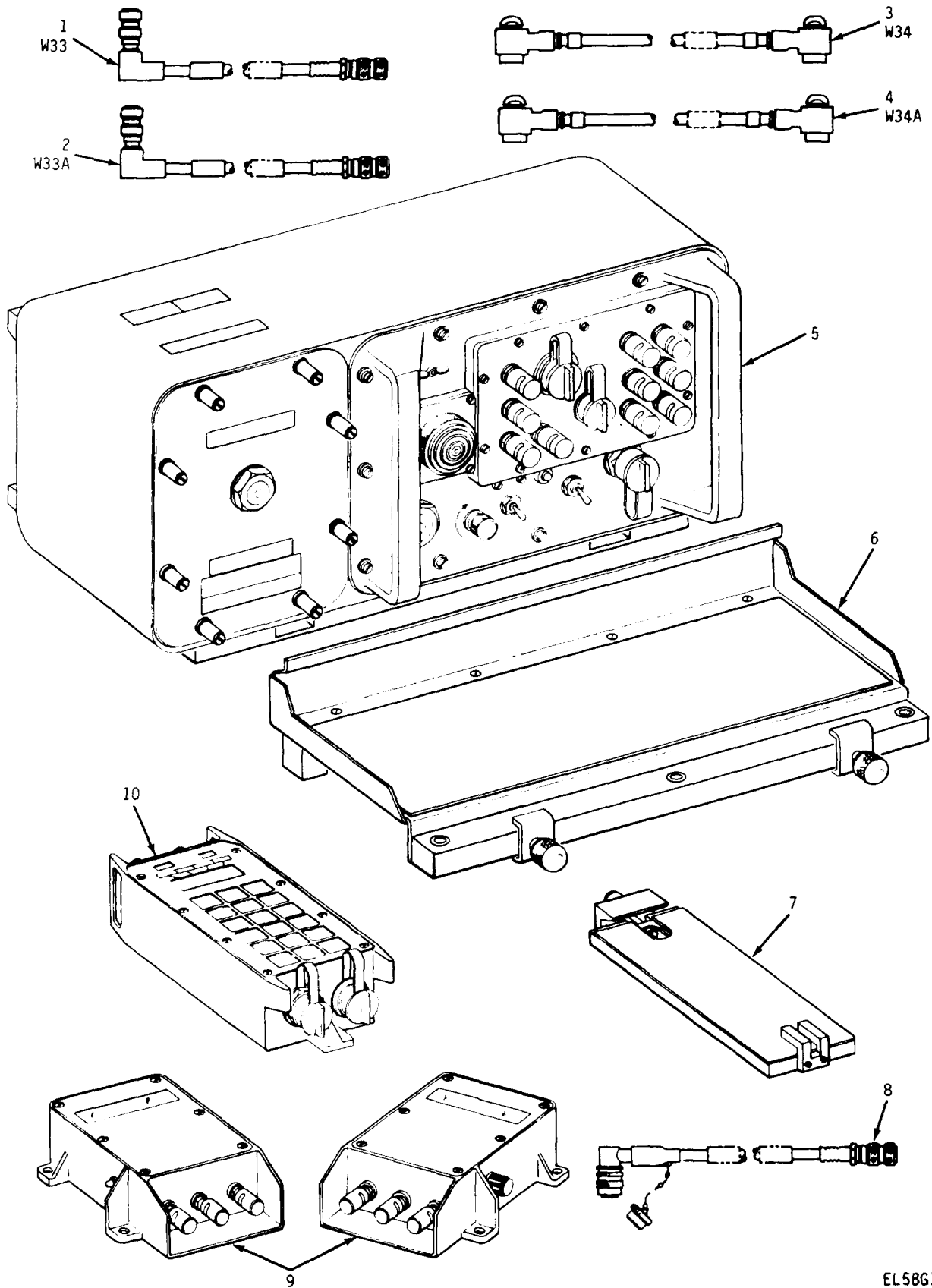
Figure 33. Data Display Group, Gun Direction OD-144(V)/GYK-29(V)
