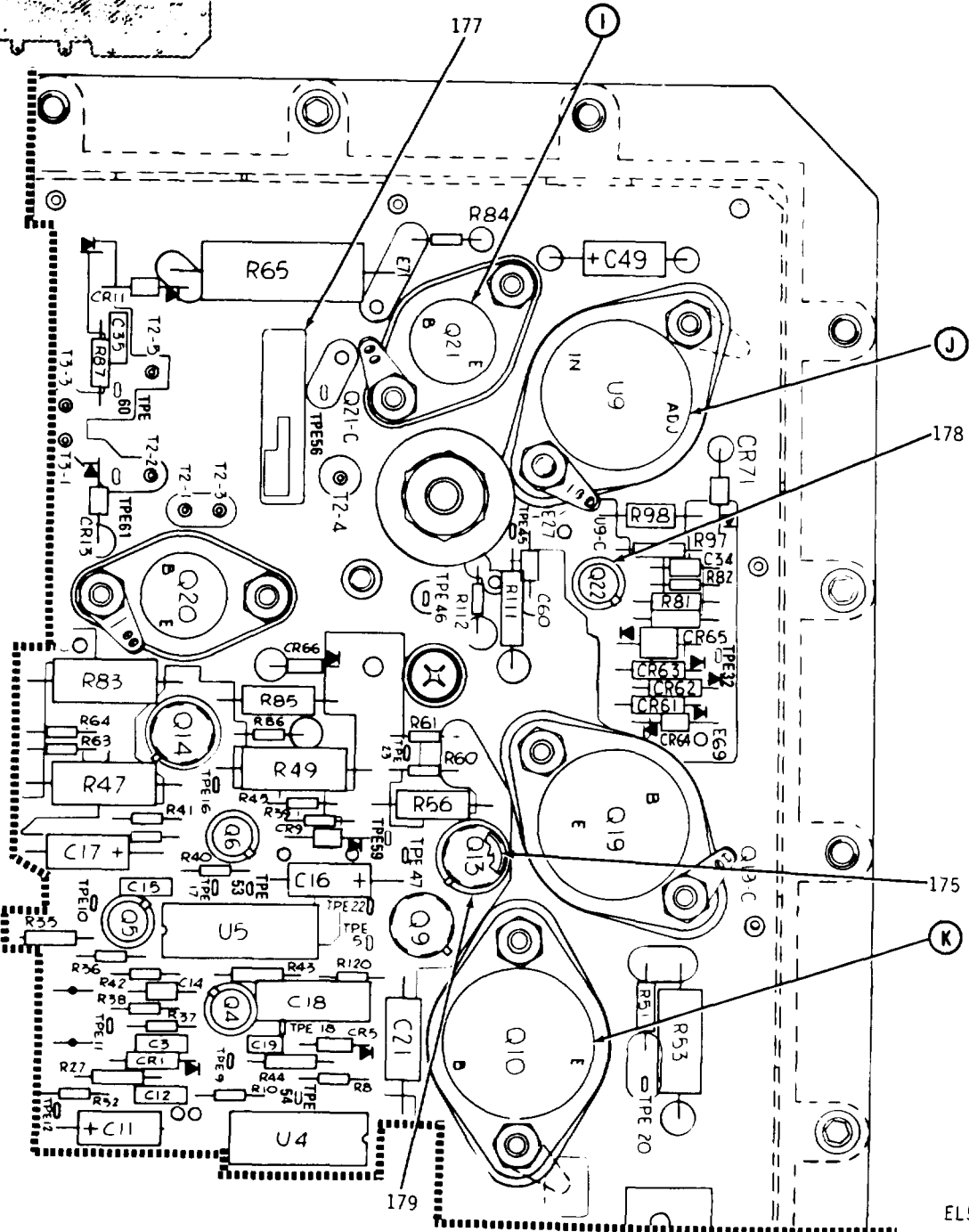
Figure 14. LVPS Main Board Assembly (Sheet 3 of 10)
