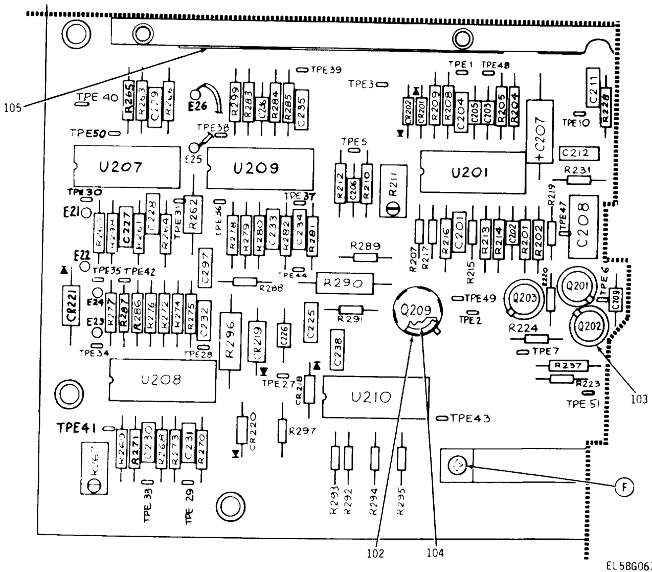
Figure 15. LVPS Backup Board Assembly (Sheet 3 of 6)
