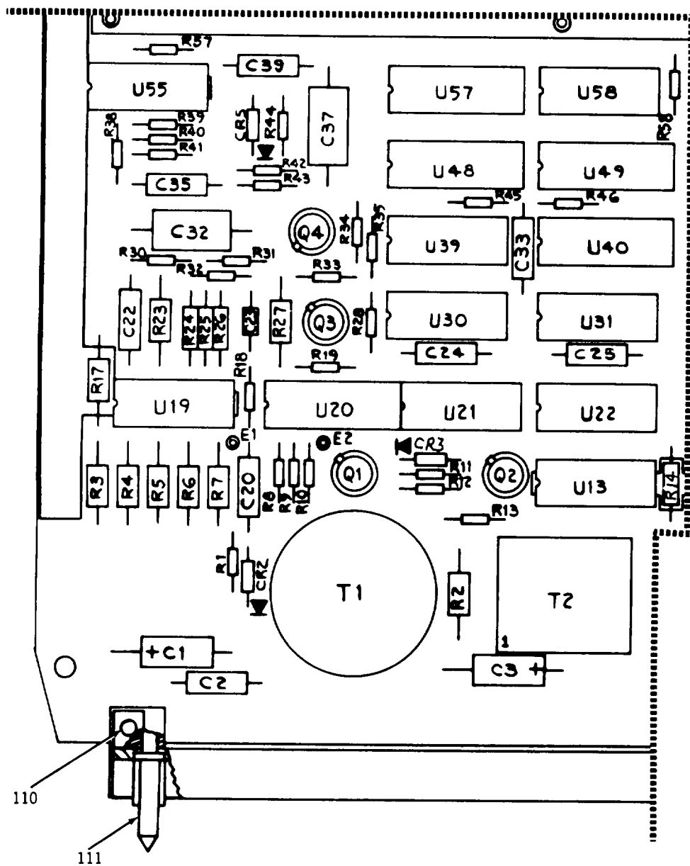
Figure 7. Gun Display Unit Interface Assembly (Sheet 4 of 5)
