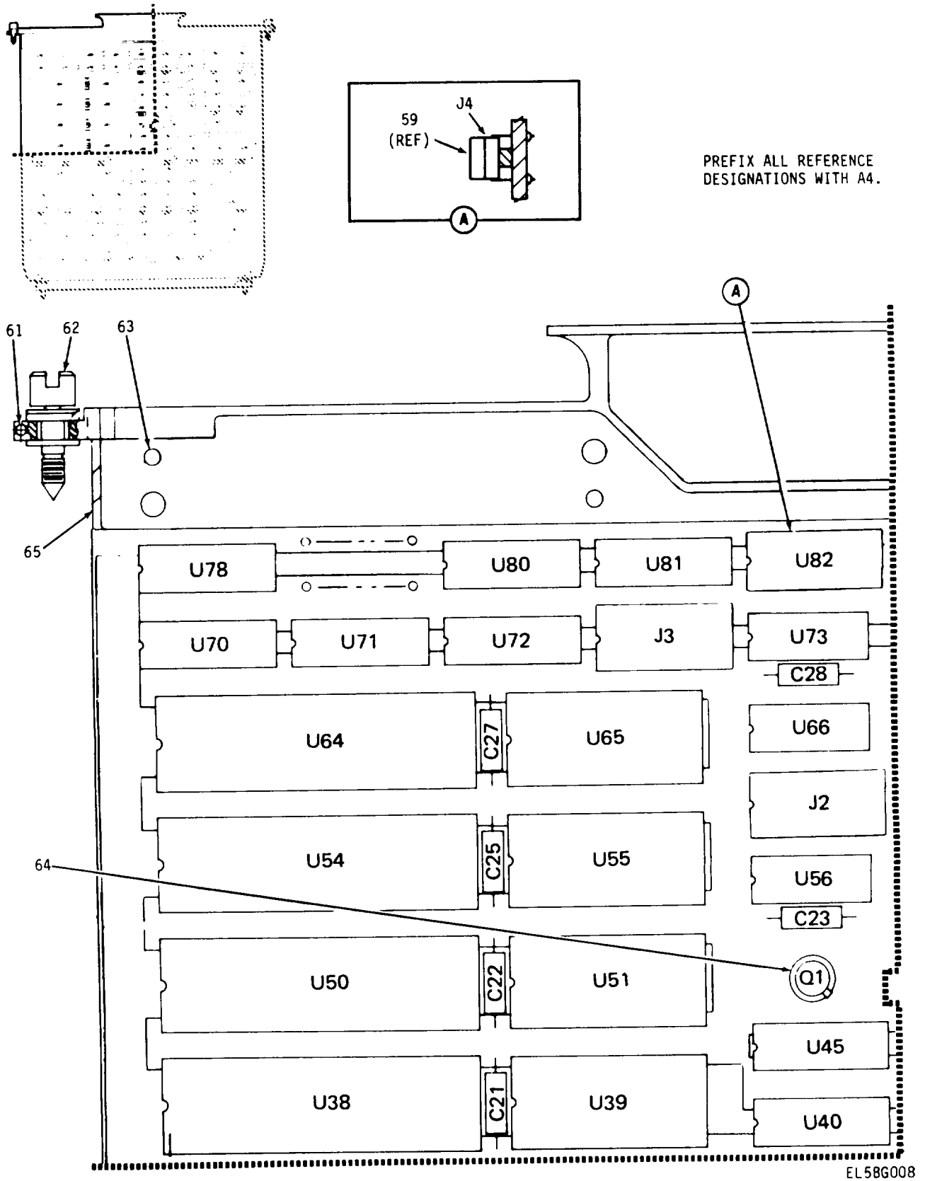
Figure 4. Central Processor Assembly (Sheet 1 of 5)
