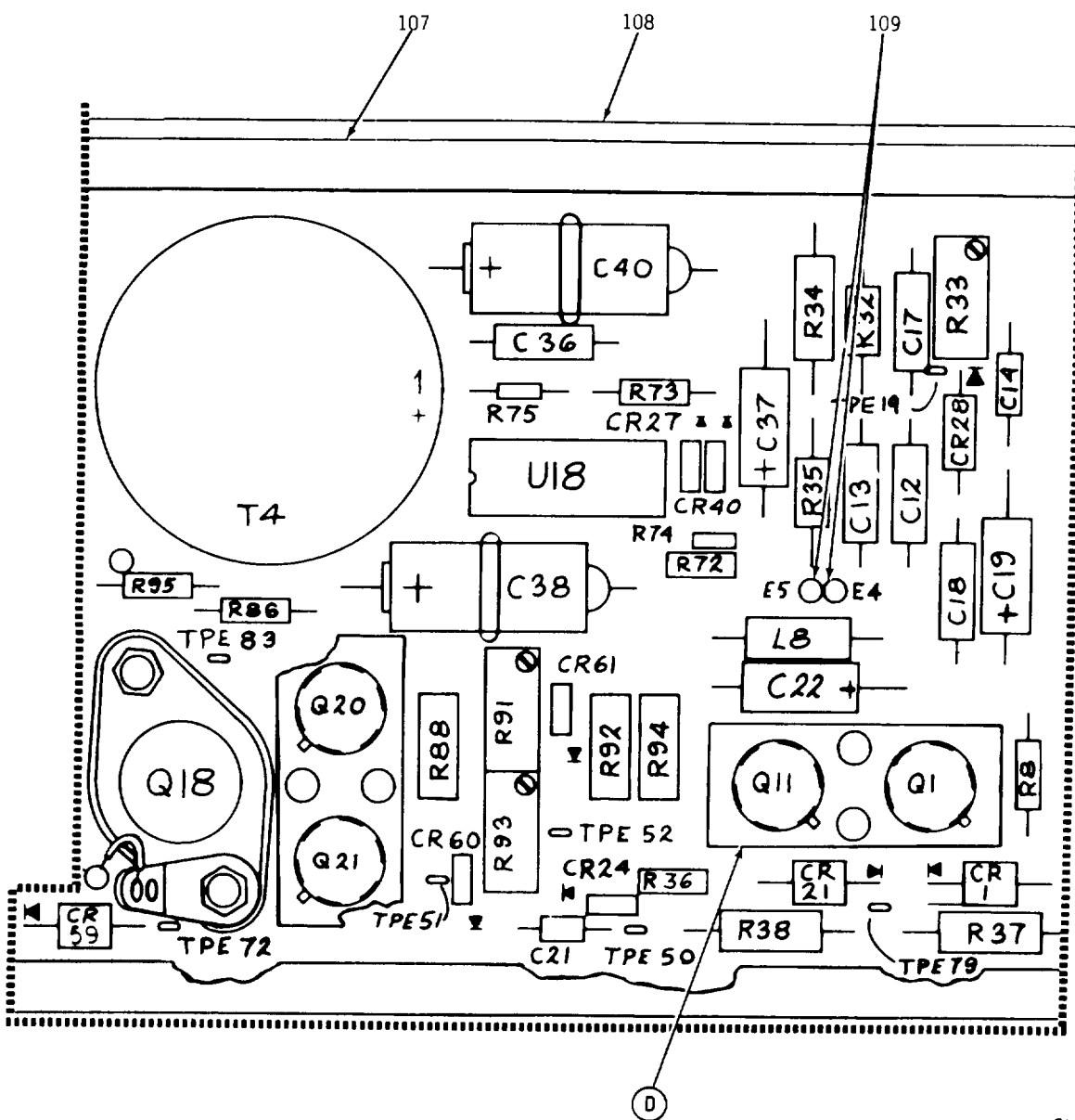
Figure 18. Interface Board Assembly (Sheet 2 of 9)
