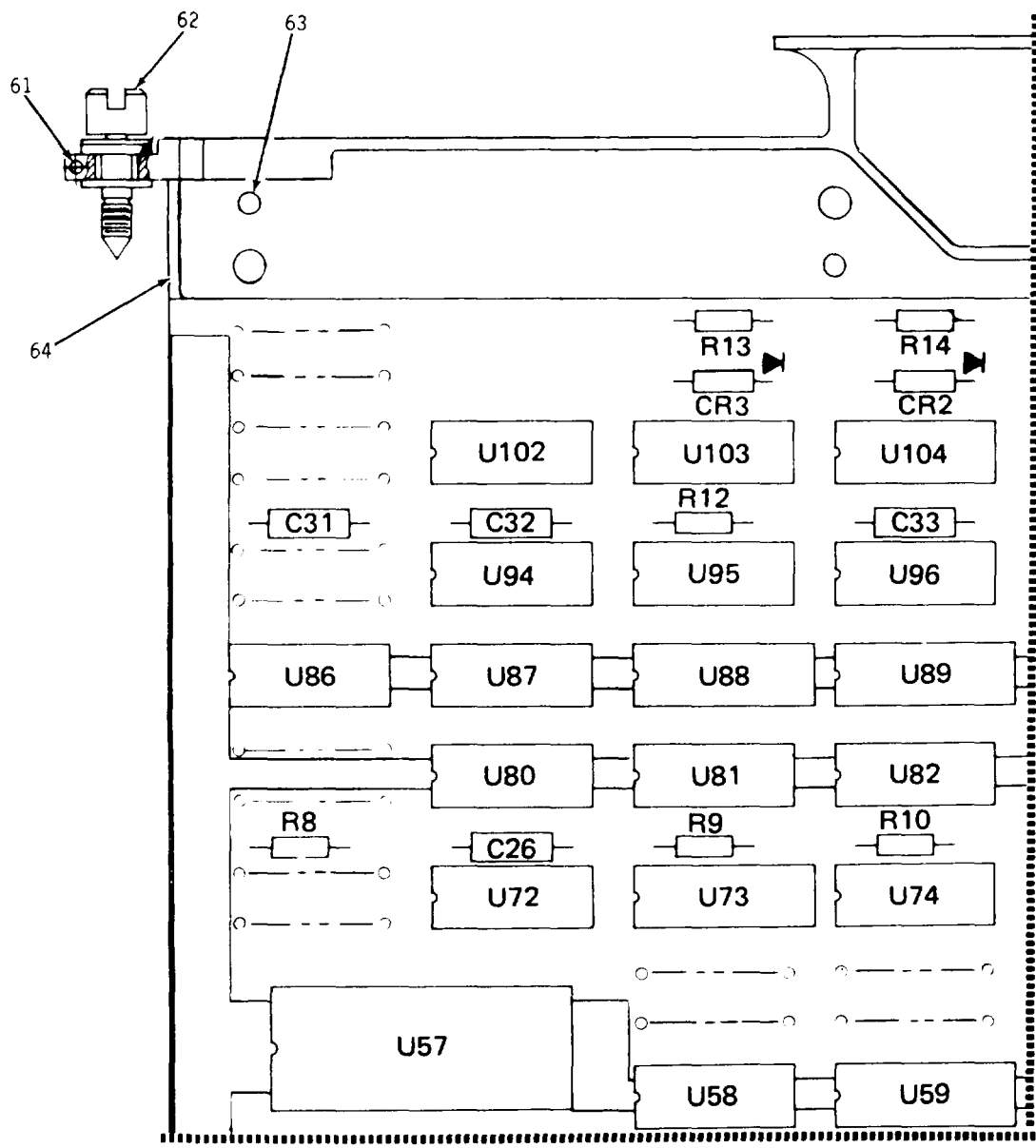
Figure 24. Central Processor Interface Assembly (Sheet 1 of 5)
