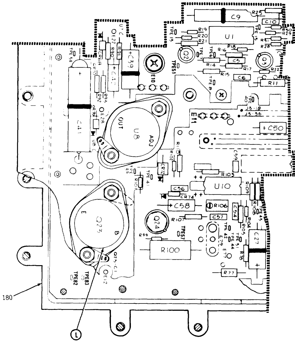
Figure 14. LVPS Main Board Assembly (Sheet 4 of 10)
