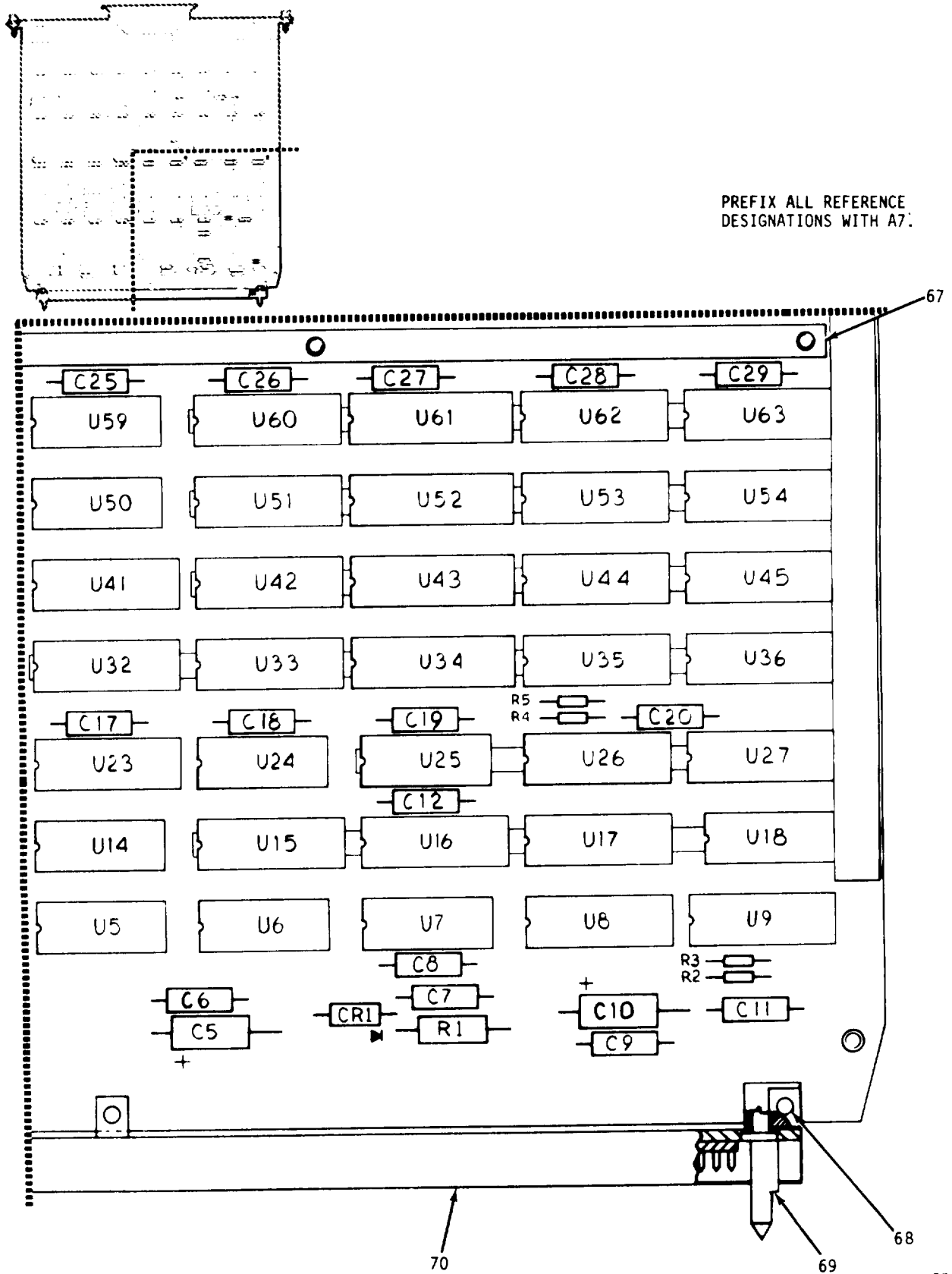
Figure 6. Interface Data Controller 2 Assembly (sheet 3 of 5)
