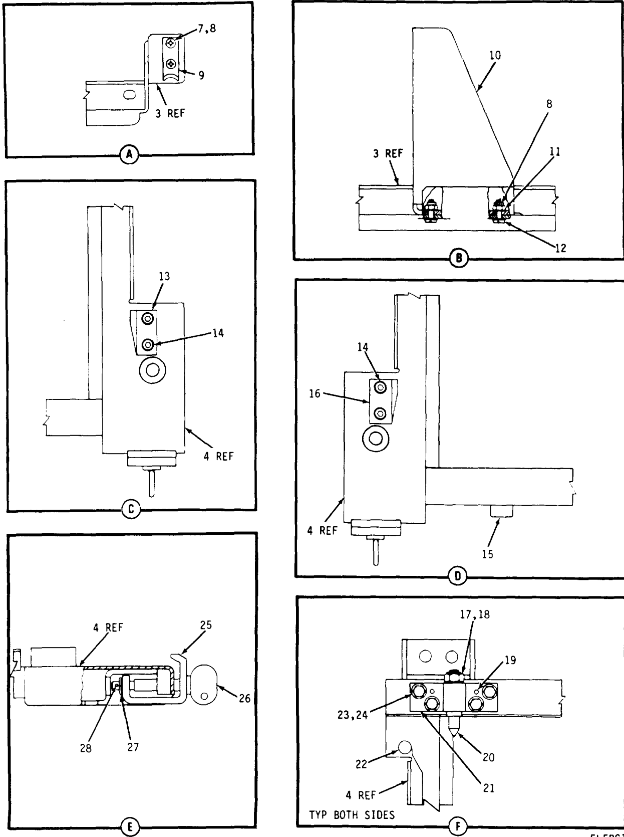
Figure 32. Mounting Base, Computer Gun Direction MT-4938/GYK-29(V) (Sheet 2 of 5)
