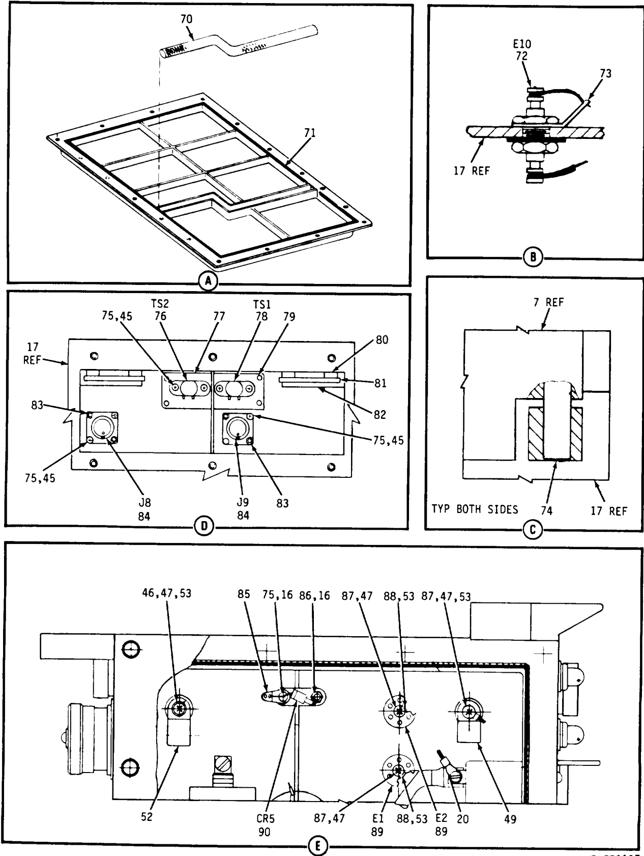
Figure 30. Power Distribution Unit (Sheet 4 of 5)
