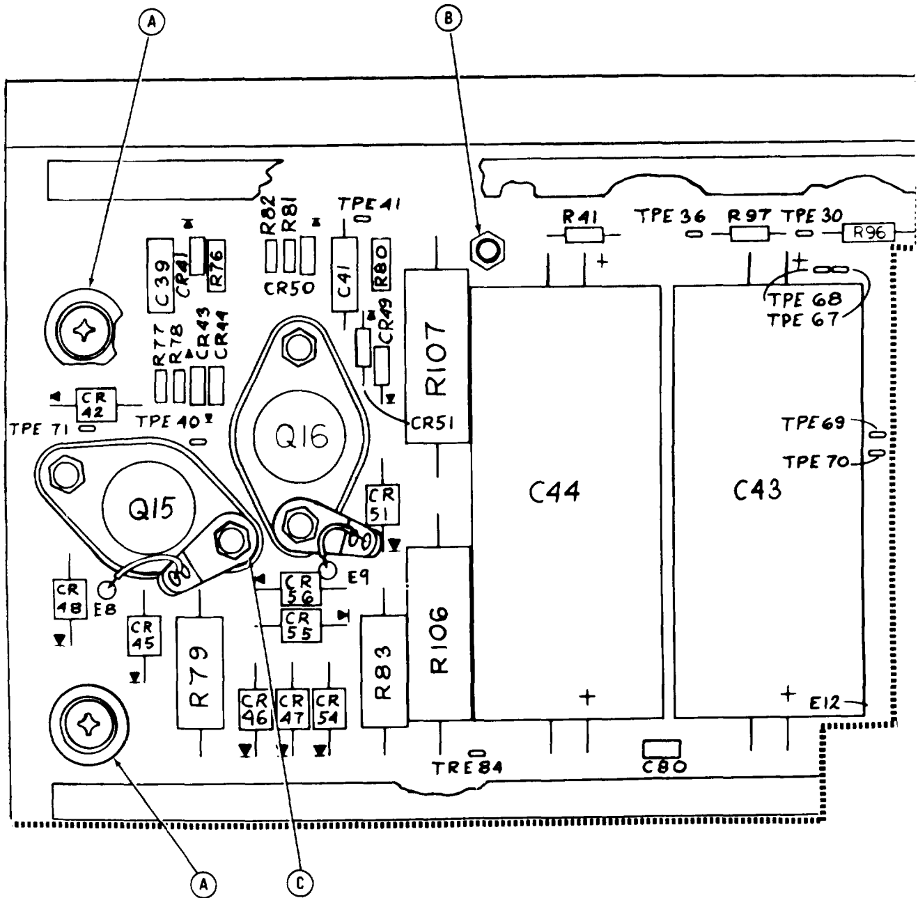
Figure 18. Interface Board Assembly (Sheet 1 of 9)
