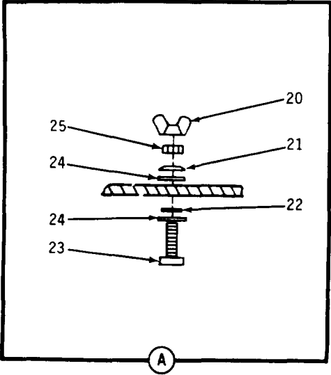
Figure 44. Power Supply Unit Chassis Assembly (Sheet 1 of 4)
