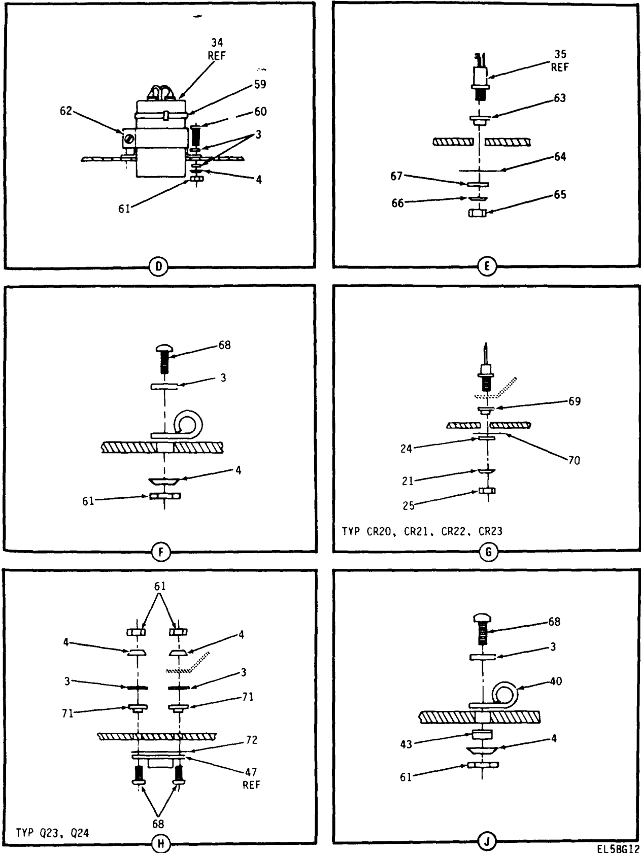
Figure 44. Power Supply Unit Chassis Assembly (Sheet 4 of 4)
