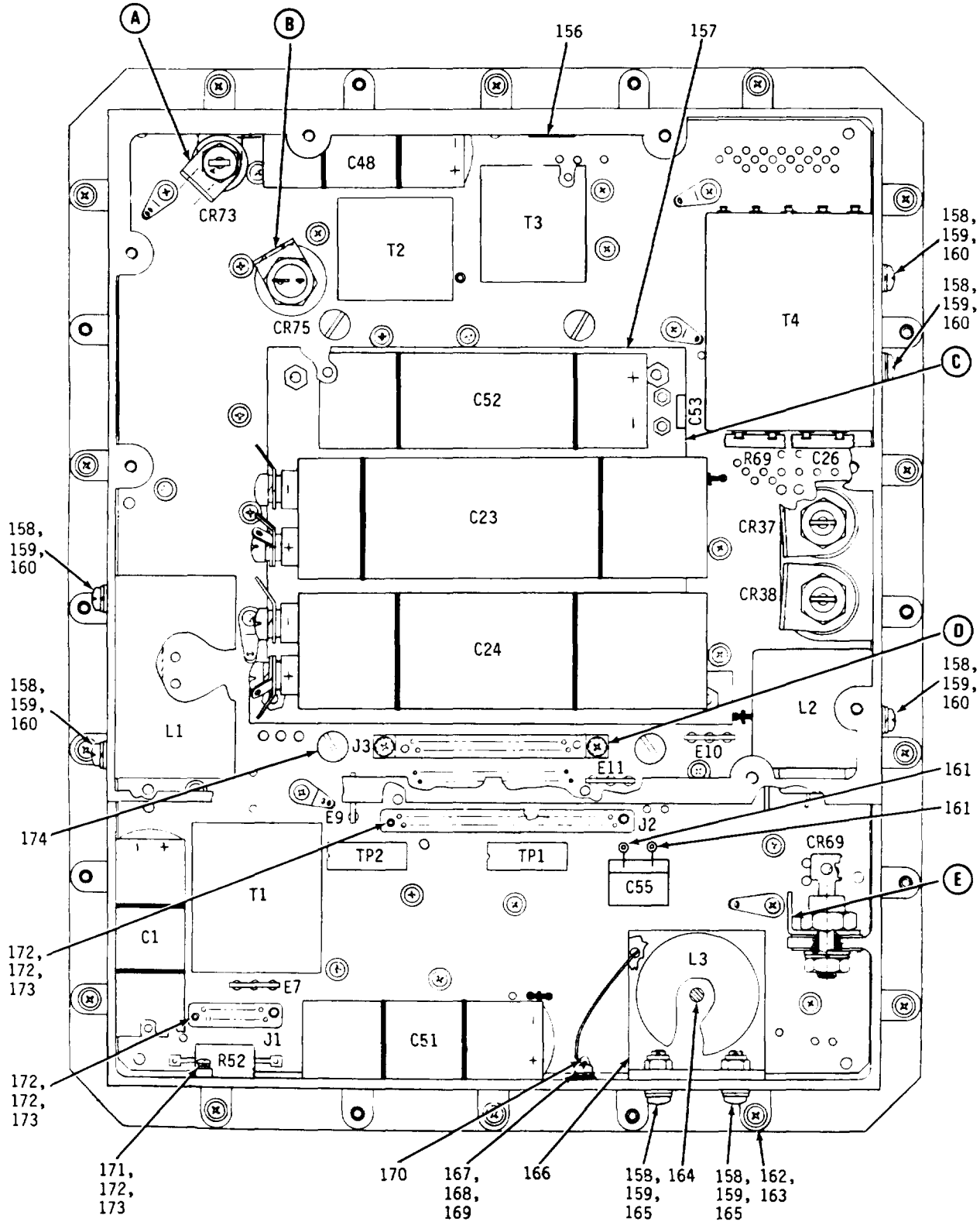
Figure 14. LVPS Main Board Assembly (Sheet 1 of 10)
