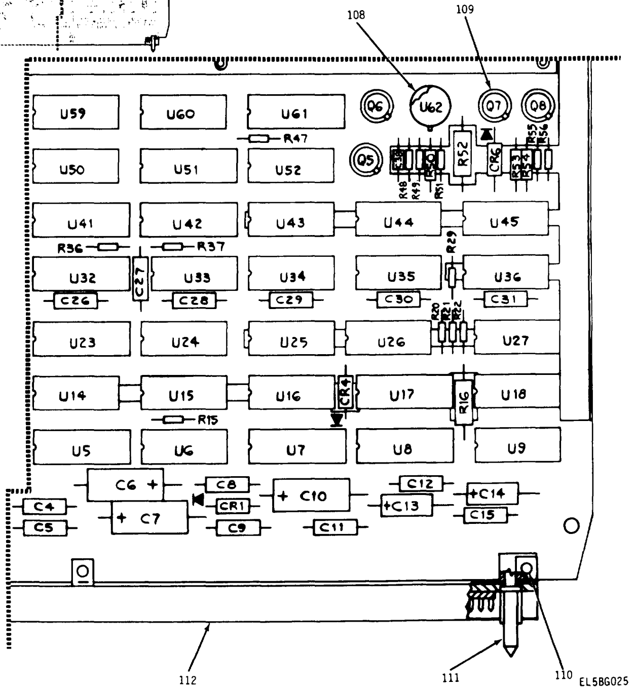
Figure 7. Gun Display Unit Interface Assembly (Sheet 3 of 5)
