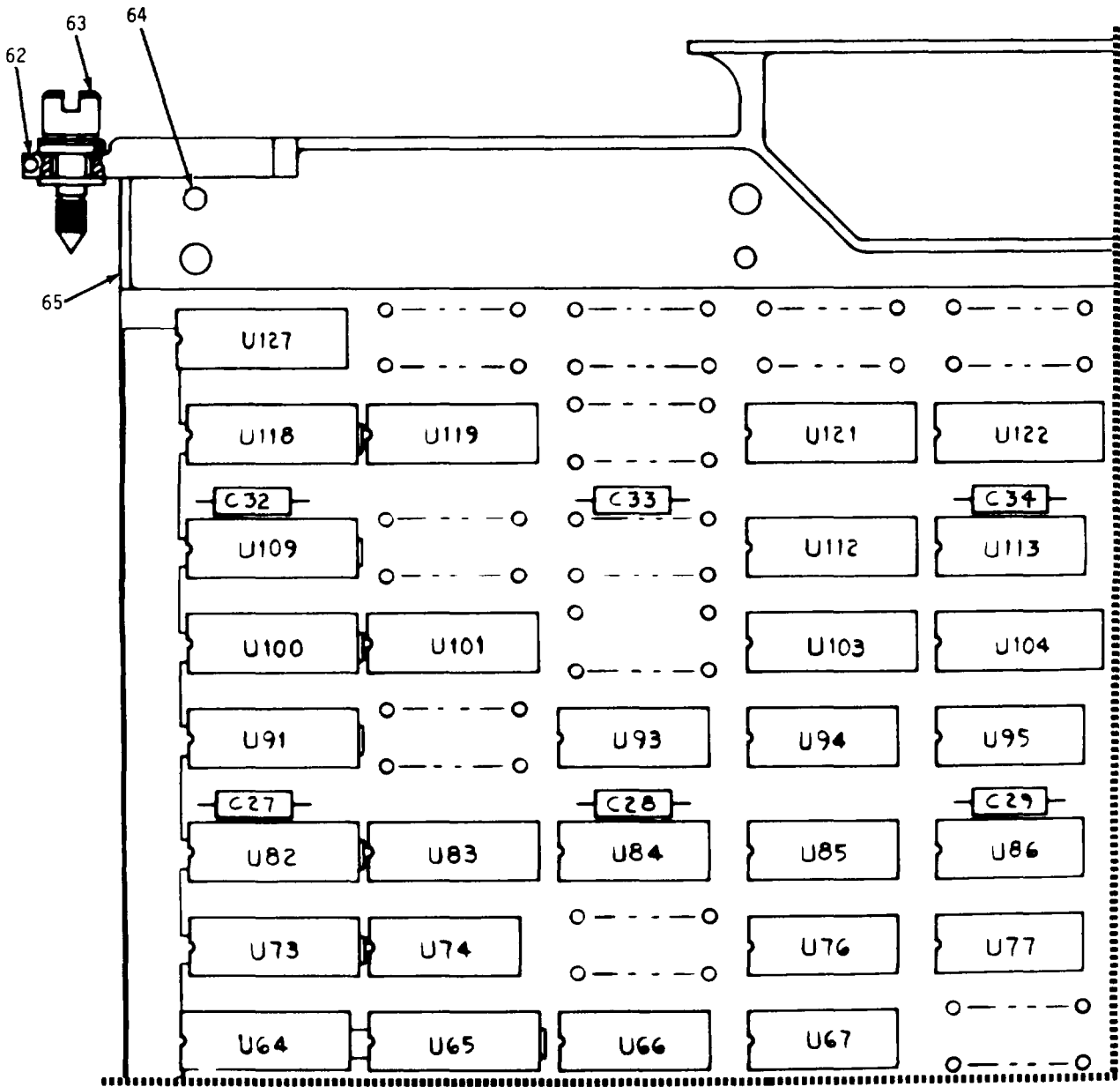
Figure 12. Symbol Generator Assembly (Sheet 1 of 5)
