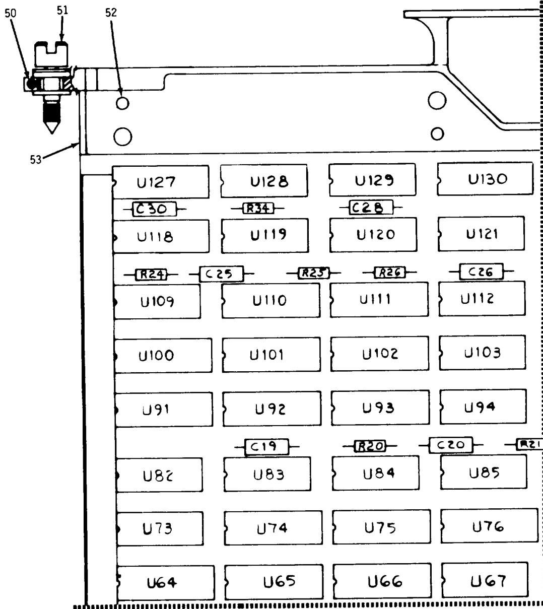
Figure 8. Communication Interface Assembly (Sheet 1 of 5)
