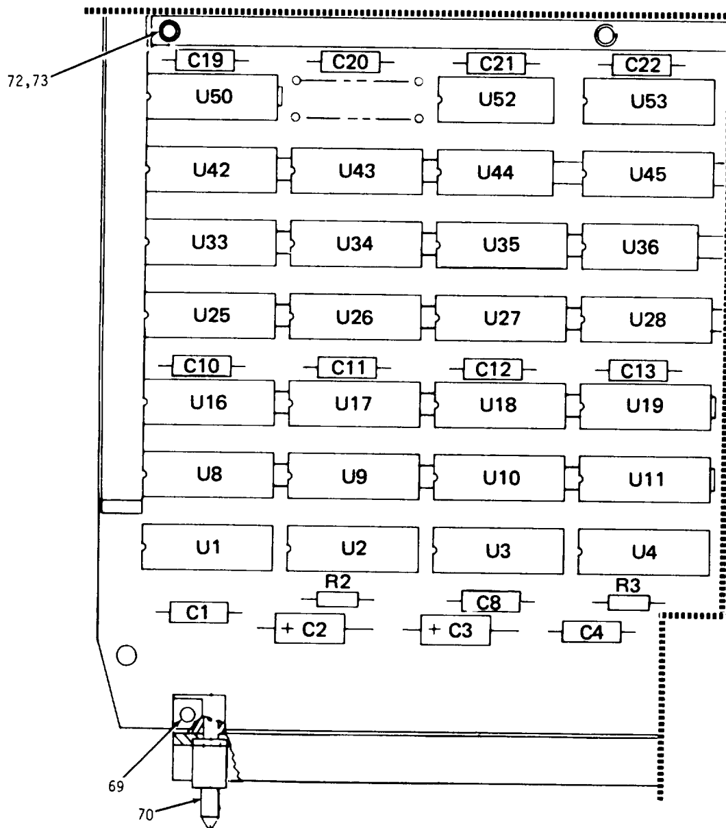
Figure 24. Central Processor Interface Assembly (Sheet 4 of 5)
