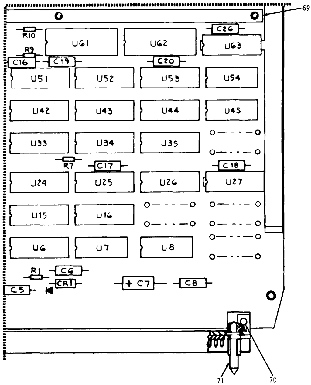
Figure 12. Symbol Generator Assembly (Sheet 3 of 5)
