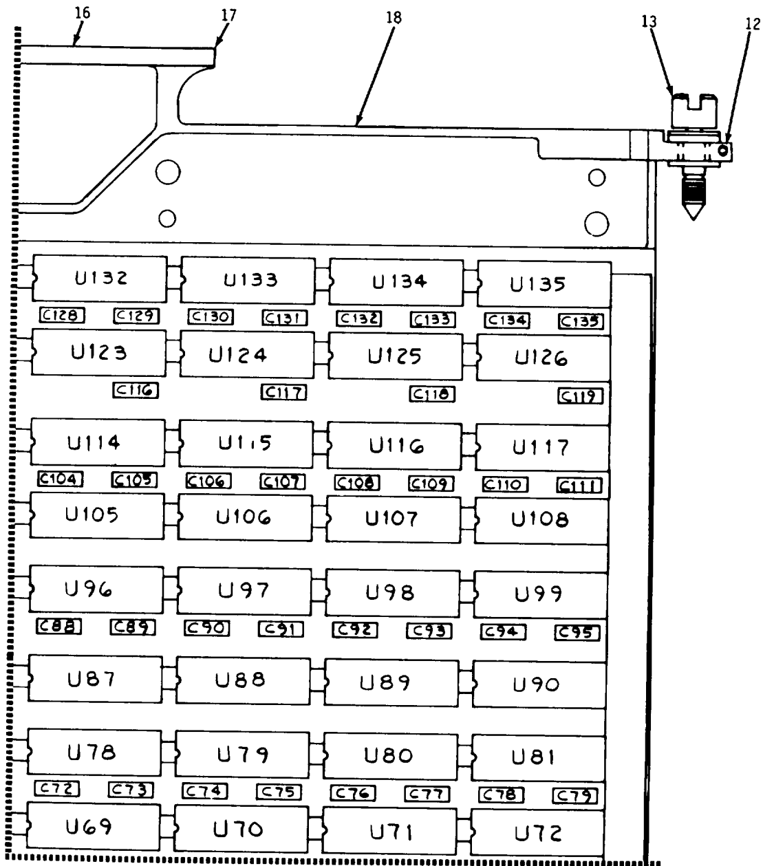
Figure 10. 65 KW Memory Assembly (Sheet 2 of 5)
