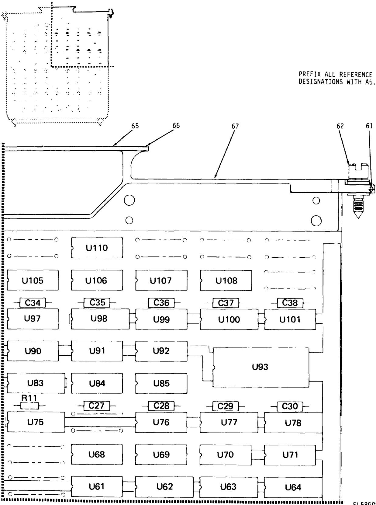
Figure 24. Central Processor Interface Assembly (Sheet 2 of 5)
