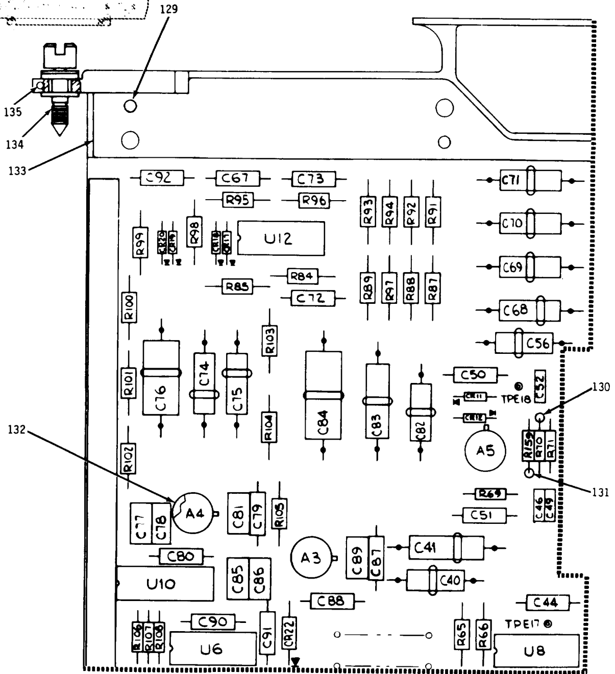
Figure 9. Communication Modem Assembly (Sheet 1 of 6)
