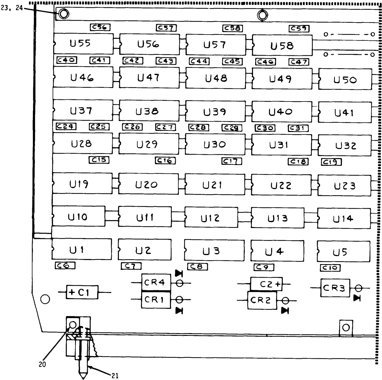
Figure 10. 65 KW Memory Assembly (Sheet 4 of 5)
