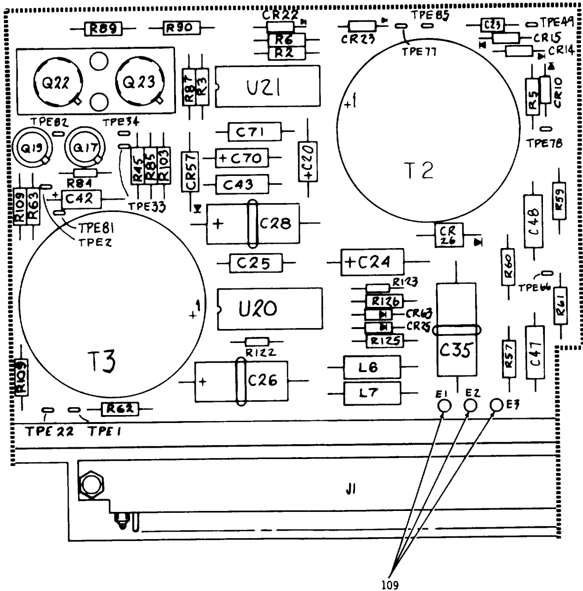
Figure 18. Interface Board Assembly (Sheet 5 of 9)
