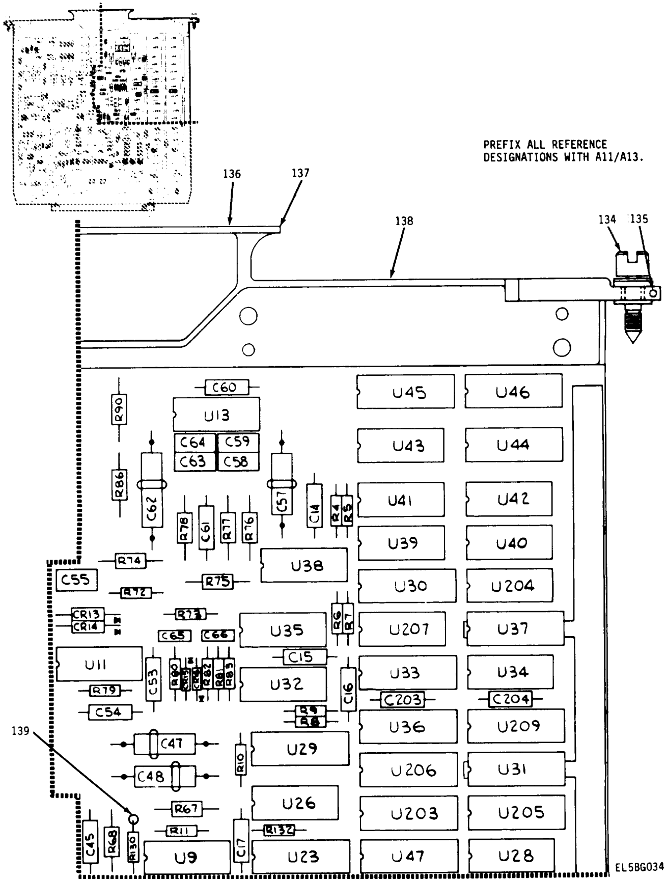
Figure 9. Communication Modem Assembly (Sheet 2 of 6)
