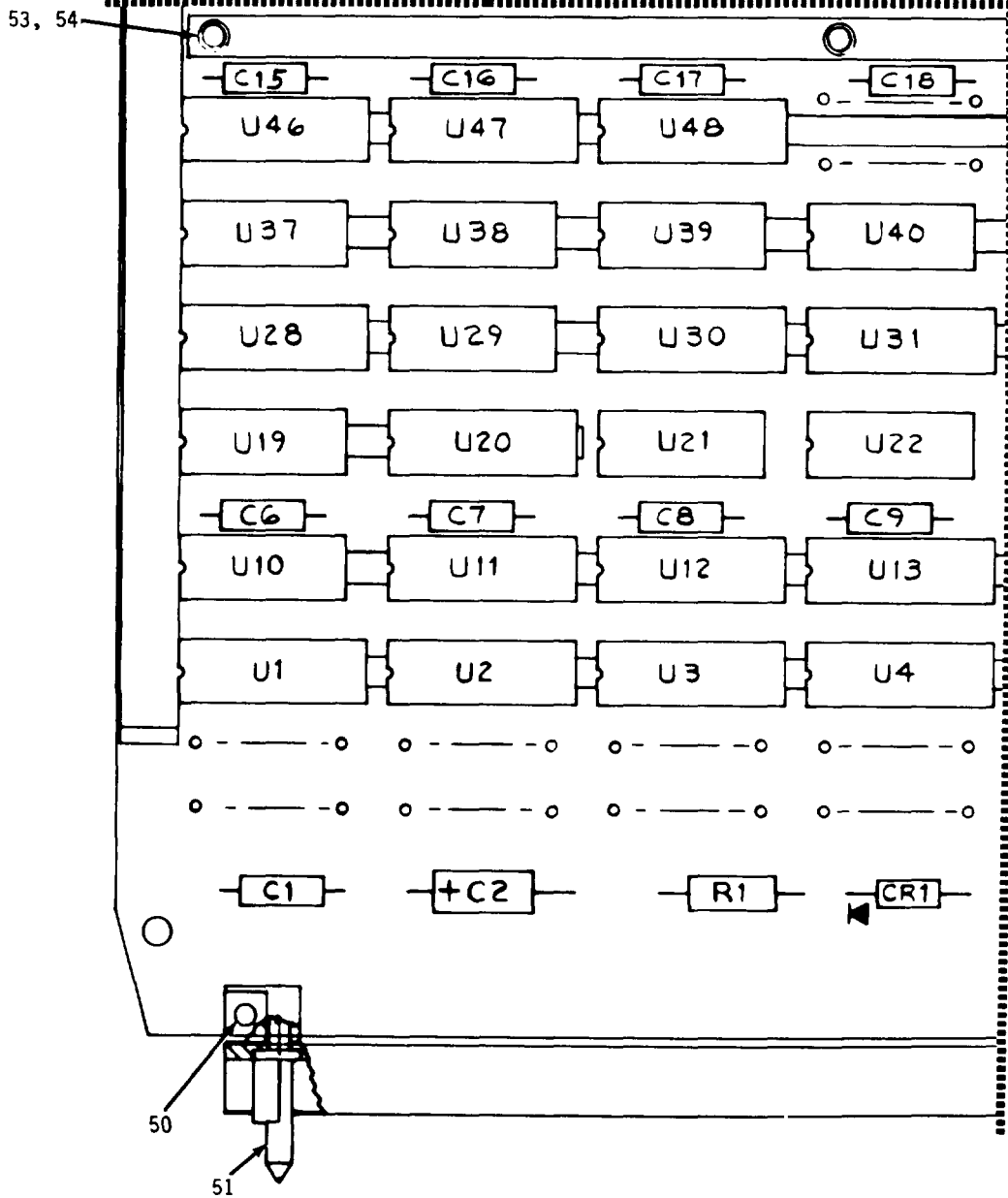
Figure 11. Memory Control Assembly (Sheet 4 of 5)
