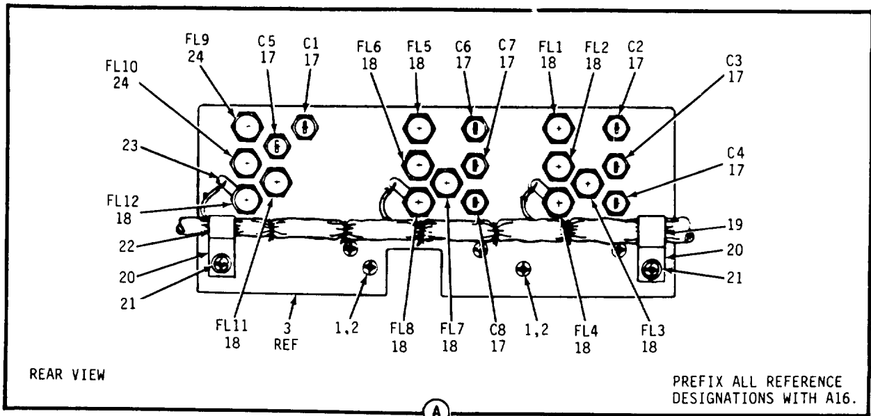
Figure 27. Comm Channel Filter Assembly (Sheet 1 of 2)
