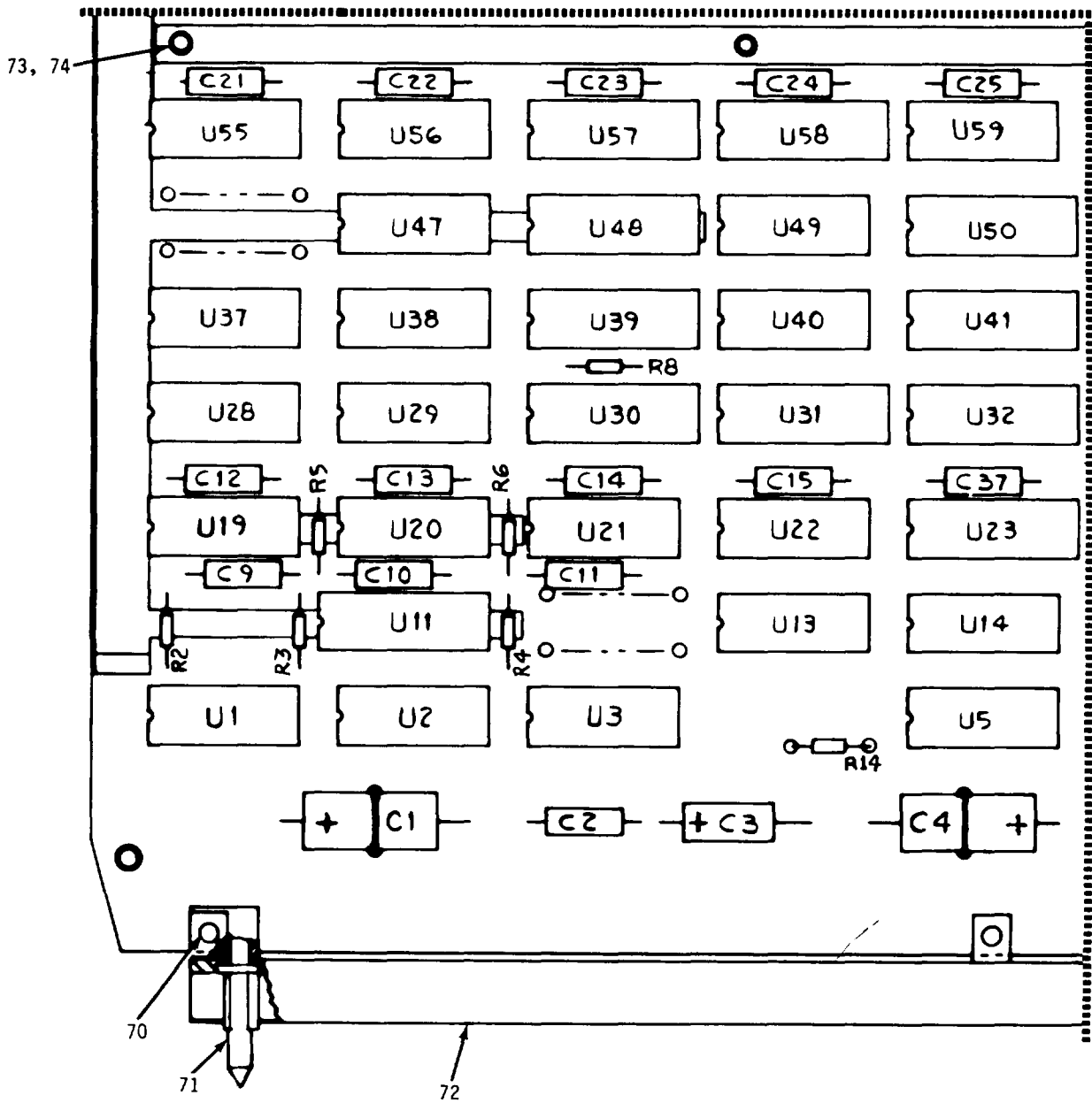
Figure 12. Symbol Generator Assembly (Sheet 4 of 5)
