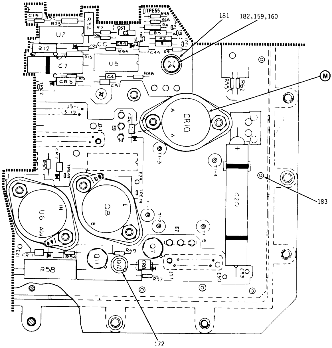
Figure 14. LVPS Main Board Assembly (Sheet 5 of 10)
