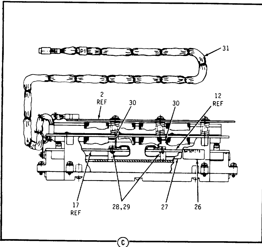
Figure 17. Plasma Panel Assembly (Sheet 2 of 3)
