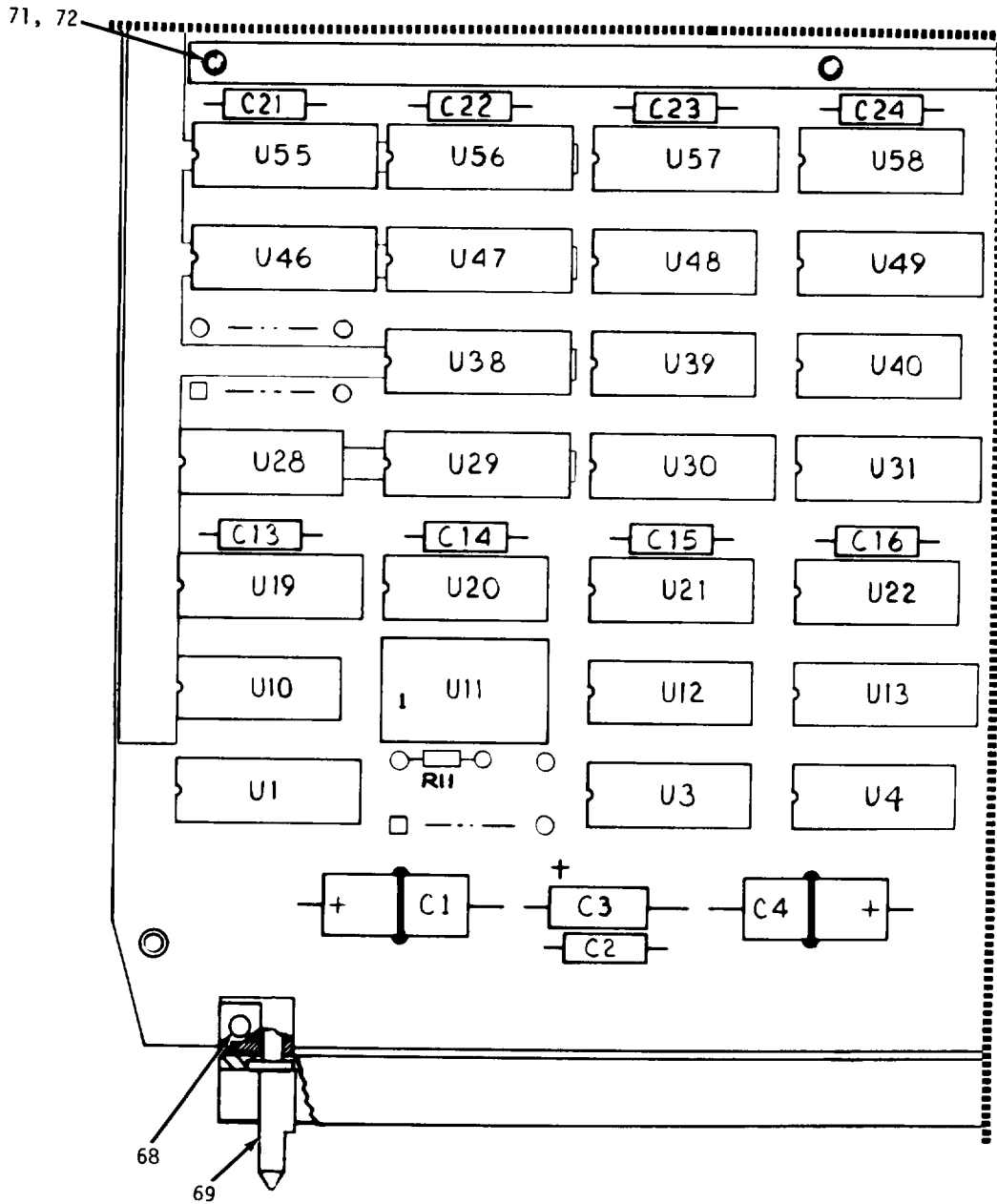
Figure 6. Interface Data Controller 2 Assembly (Sheet 4 of 5)
