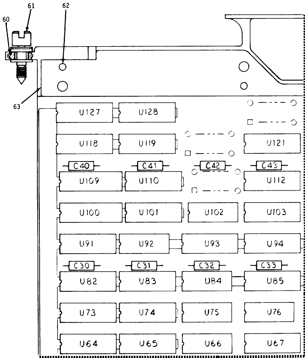
Figure 6. Interface Data Controller 2 Assembly (Sheet 1 of 5)
