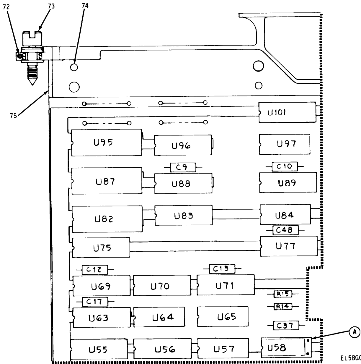
Figure 5. Interface Data Controller 1 Assembly (Sheet 1 of 5)
