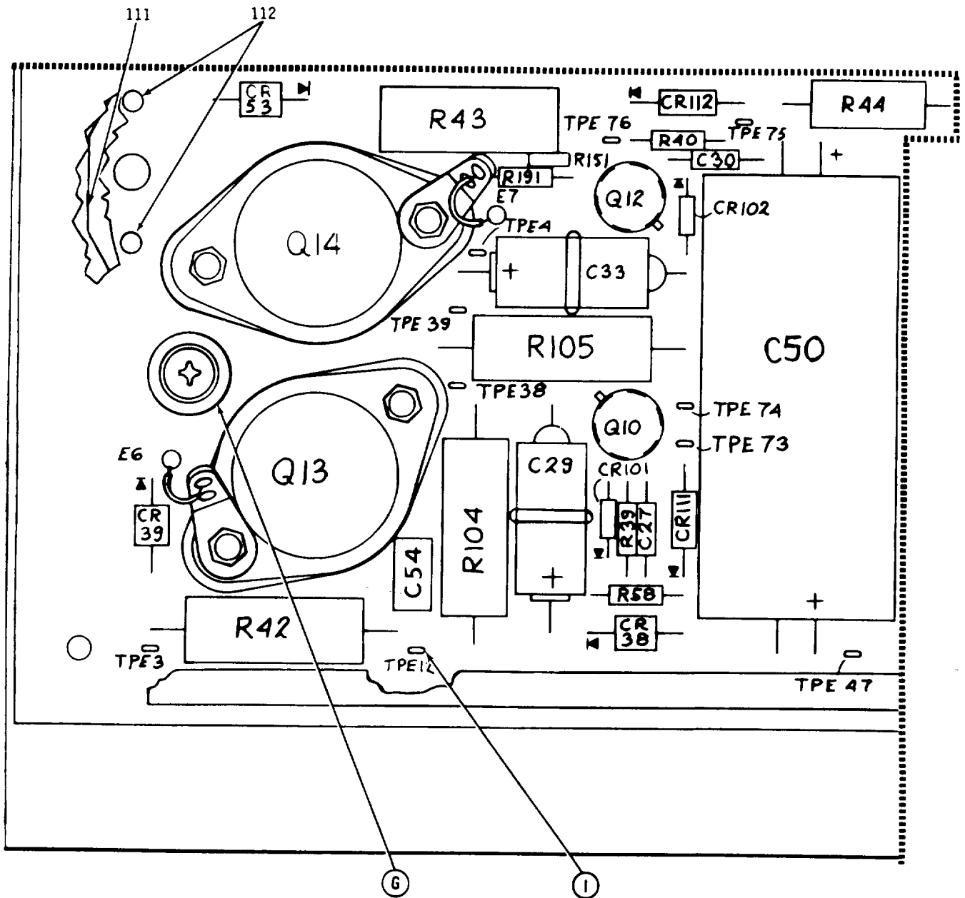
Figure 18. Interface Board Assembly (Sheet 6 of 9)
