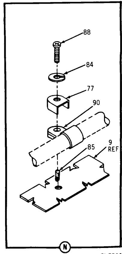
Figure 25. Housing Assembly (Sheet 5 of 7)
