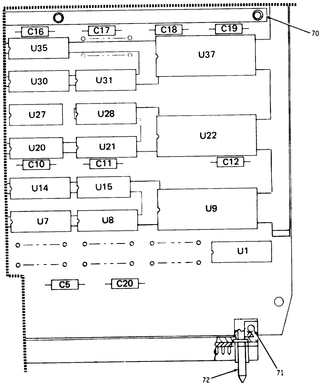
Figure 4. Central Processor Assembly (Sheet 3 of 5)
