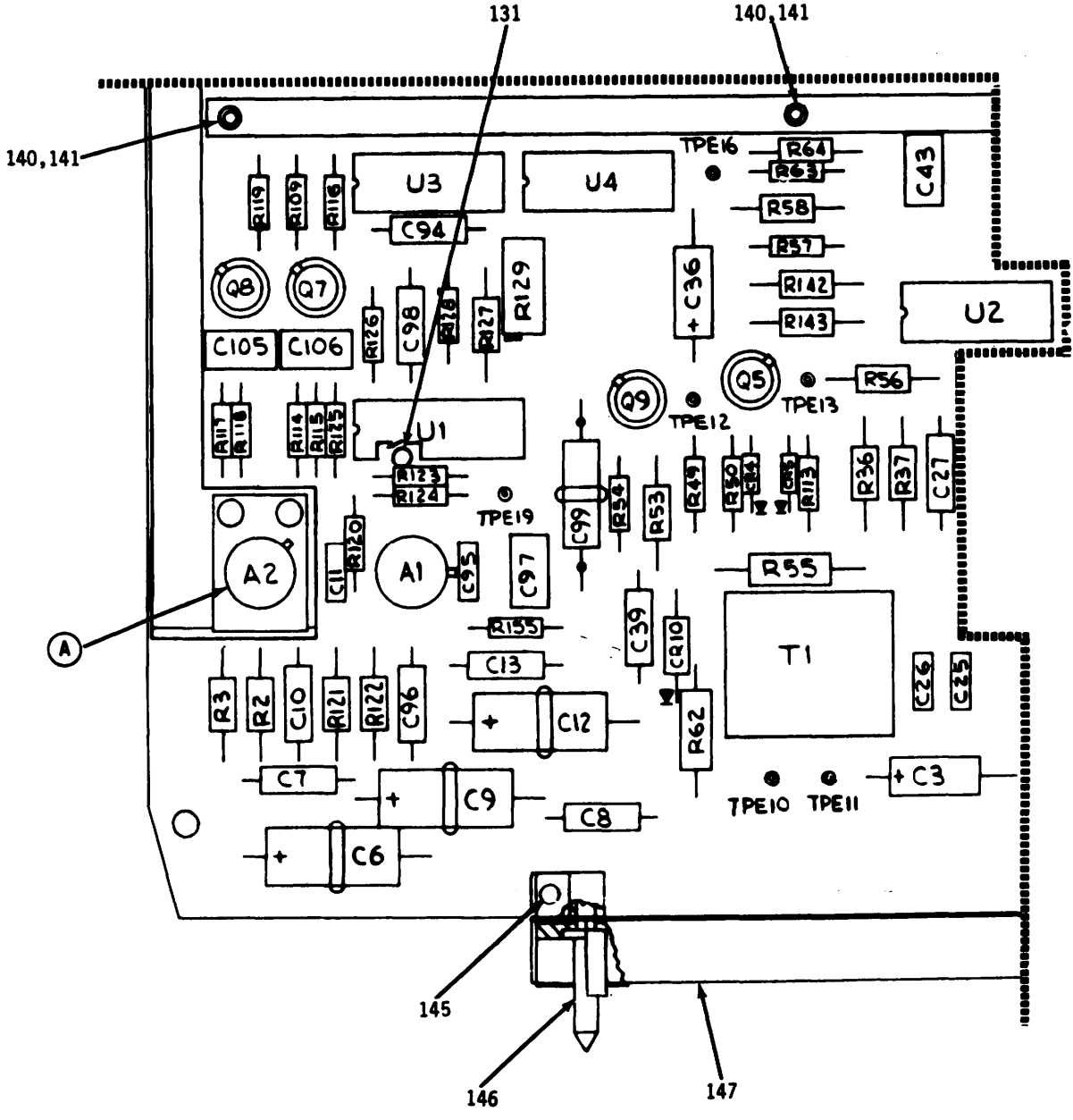
Figure 9. Communication Modem Assembly (Sheet 4 of 6)
