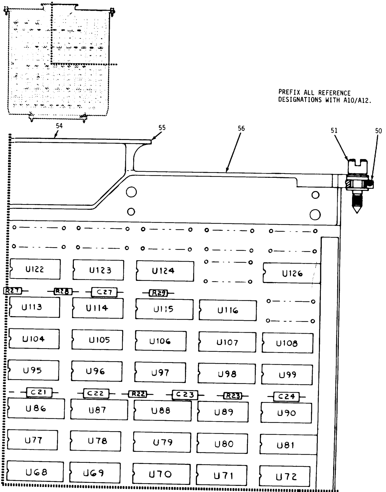
Figure 8. Communication Interface Assembly (Sheet 2 of 5)
