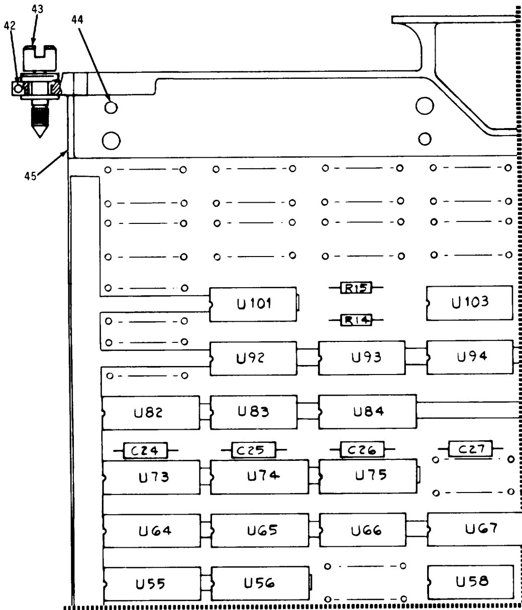
Figure 11. Memory Control Assembly (Sheet 1 of 5)
