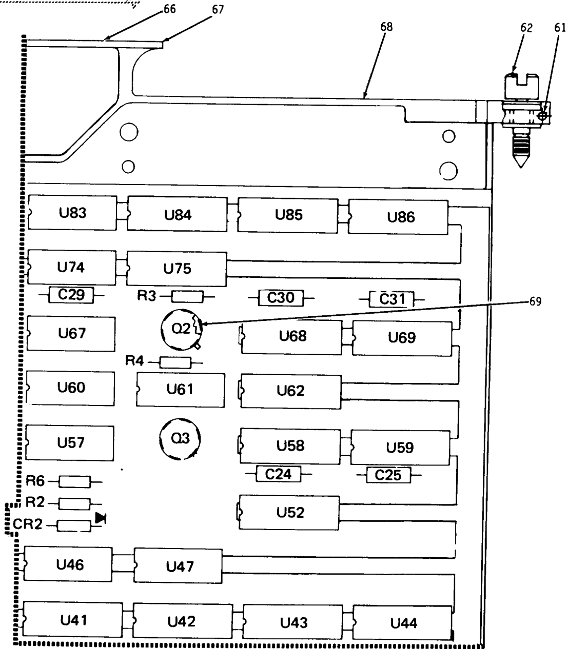
Figure 4. Central Processor Assembly (Sheet 2 of 5)
