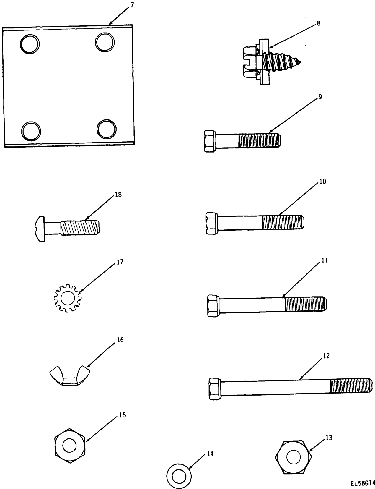
Figure 48. Mounting Kit Assembly MK-1831/GKY-29(V) (Sheet 2 of 2)
