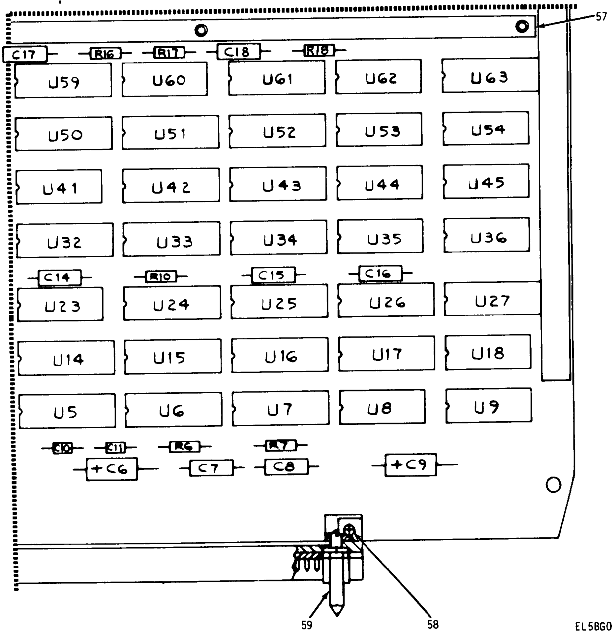
Figure 8. Communication Interface Assembly (Sheet 3 of 5)
