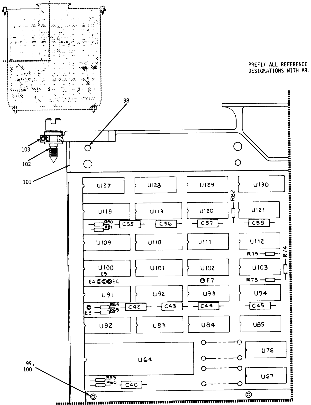
Figure 7. Gun Display Unit Interface Assembly (Sheet 1 of 5)
